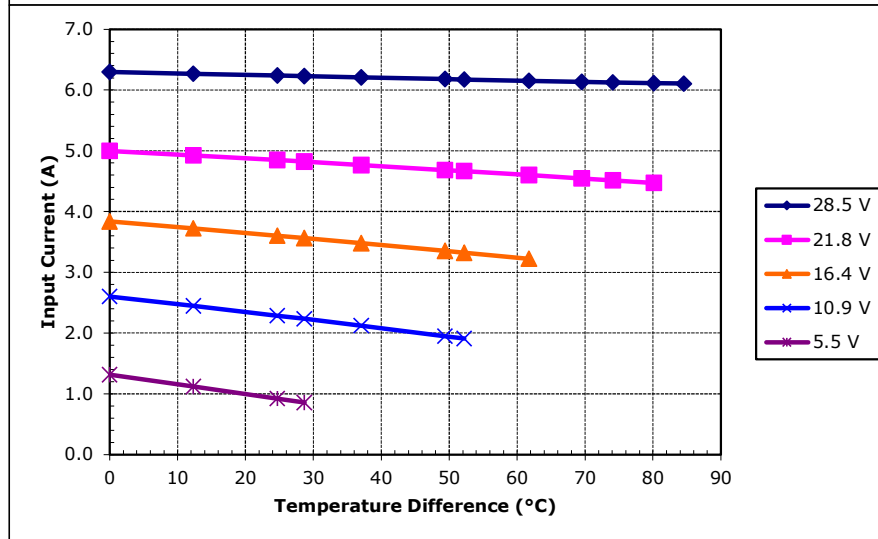
Unpotted VT-199-1.4-1.5 at a hot-side temperature of 70 °C
