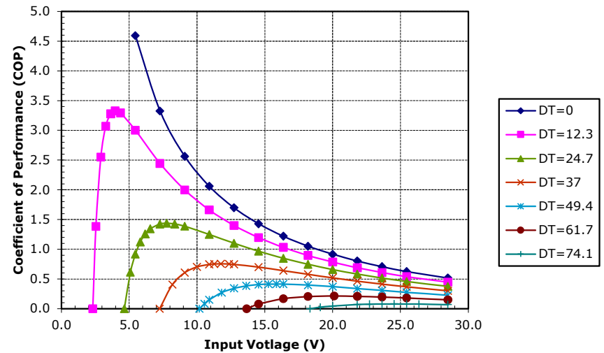
Unpotted VT-199-1.4-1.5 at a hot-side temperature of 70 °C
