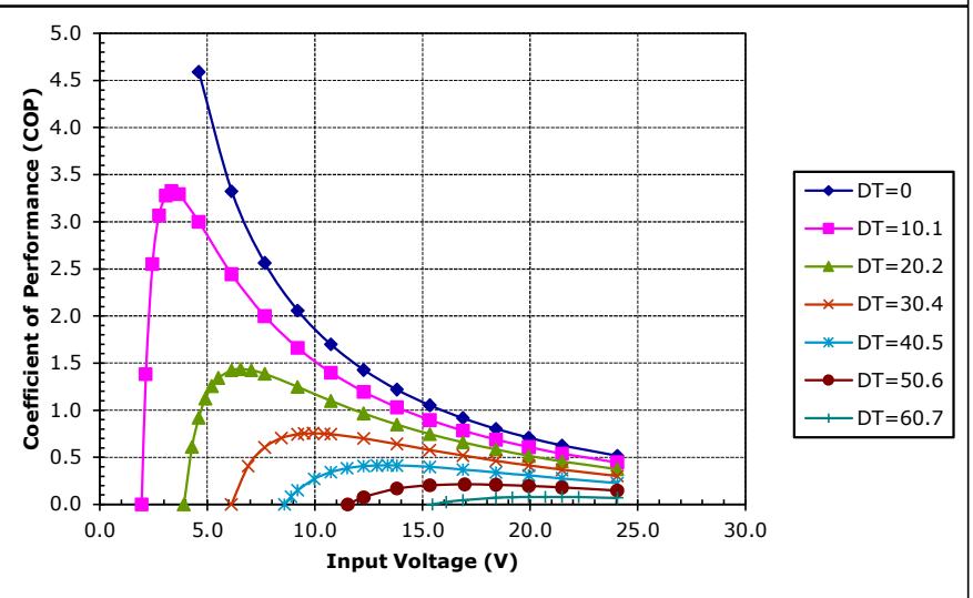
Unpotted VT-199-1.4-1.5 at a hot-side temperature of 30 °C
