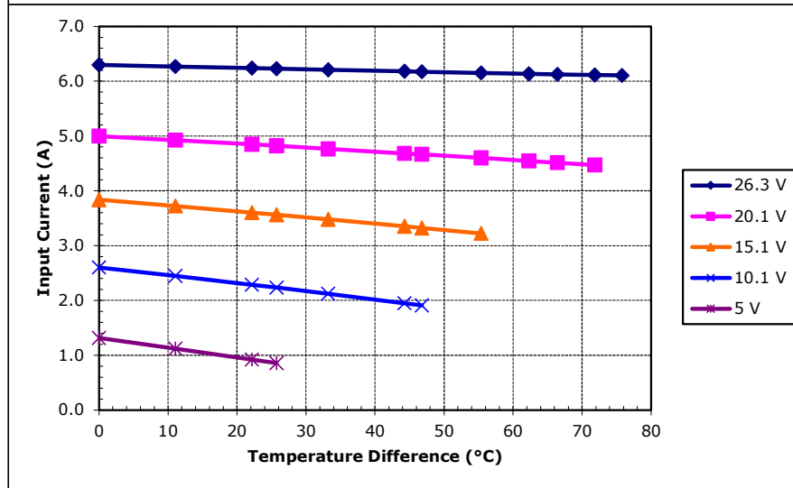
Potted VT-199-1.4-1.5 at a hot-side temperature of 50 °C
