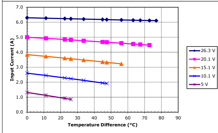
Unpotted VT-199-1.4-1.5 at a hot-side temperature of 50 °C
