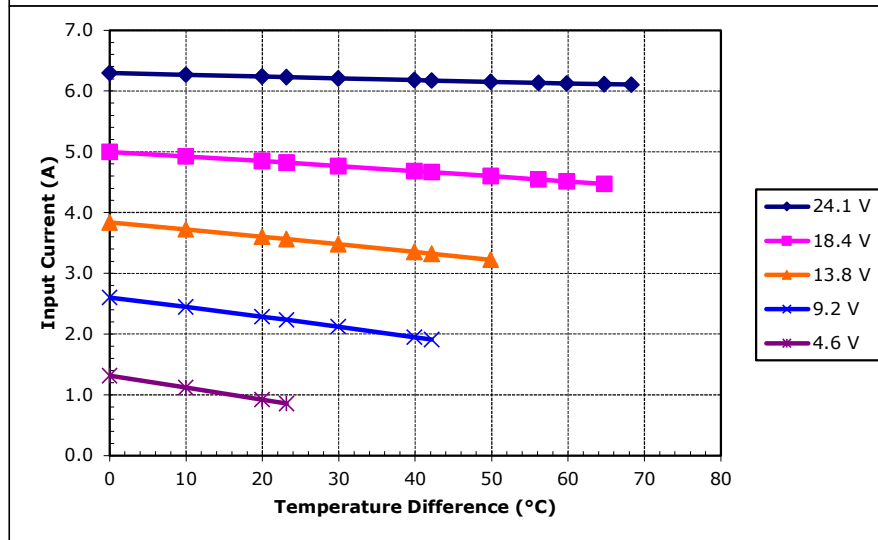
Potted VT-199-1.4-1.5 at a hot-side temperature of 30 °C
