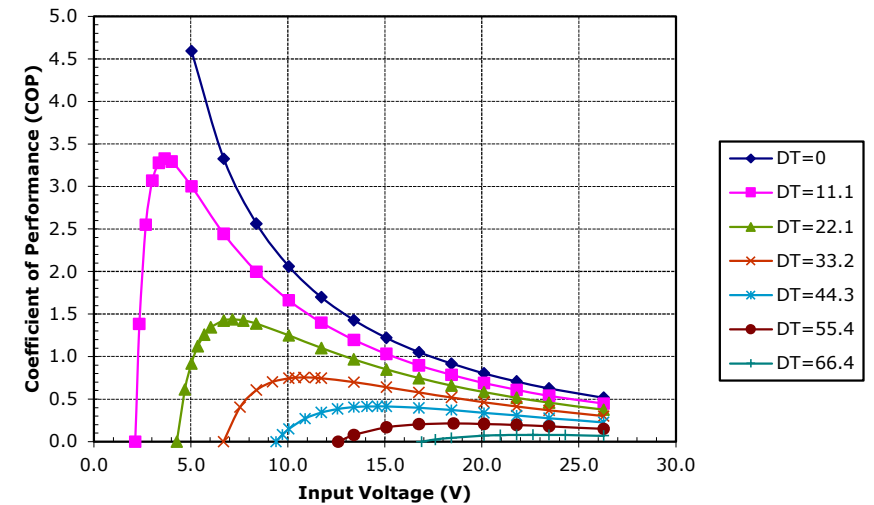
Potted VT-199-1.4-1.5 at a hot-side temperature of 50 °C
