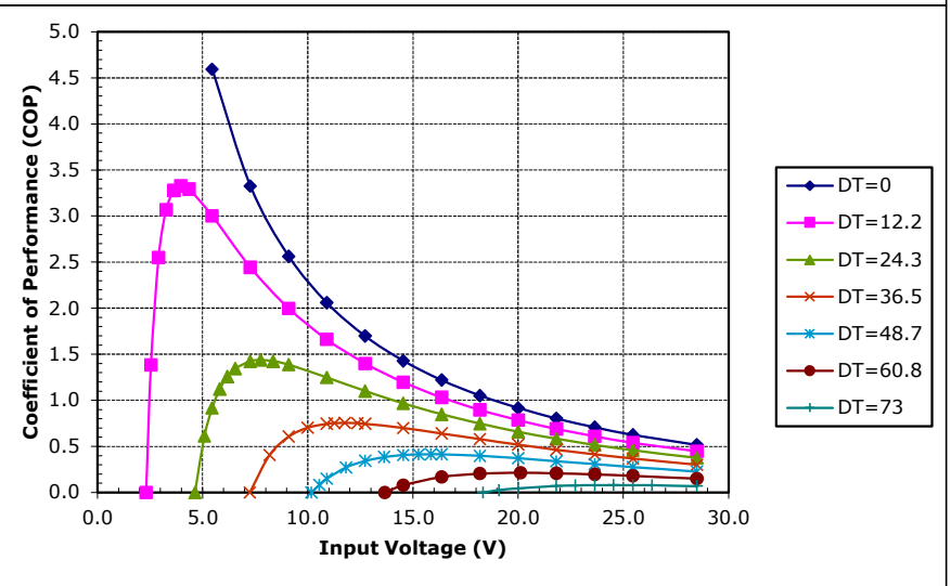
Potted VT-199-1.4-1.5 at a hot-side temperature of 70 °C
