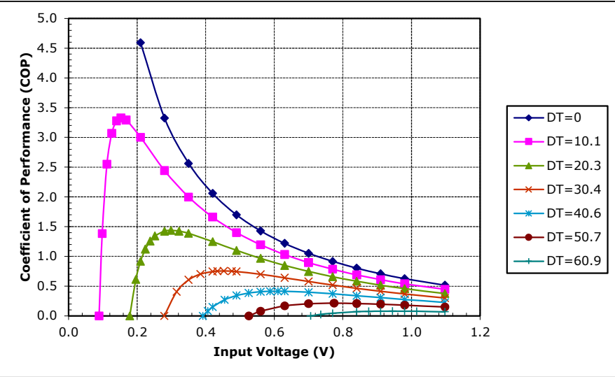
Potted TE-8-0.45-1.3 at a hot-side temperature of 50 °C
