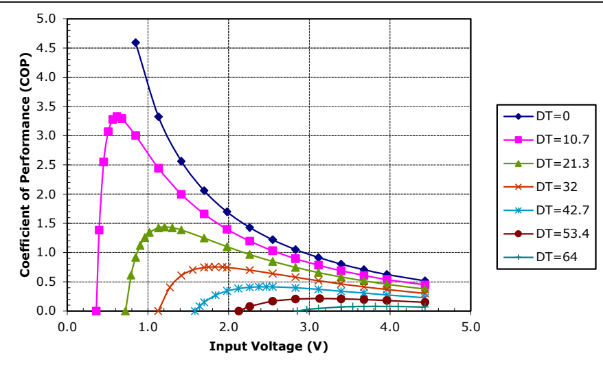
Potted TE-32-0.45-1.3 at a hot-side temperature of 50 °C
