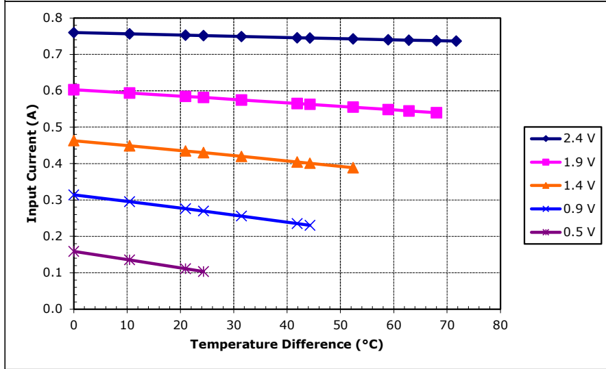
Potted TE-18-0.45-1.3 at a hot-side temperature of 50 °C
