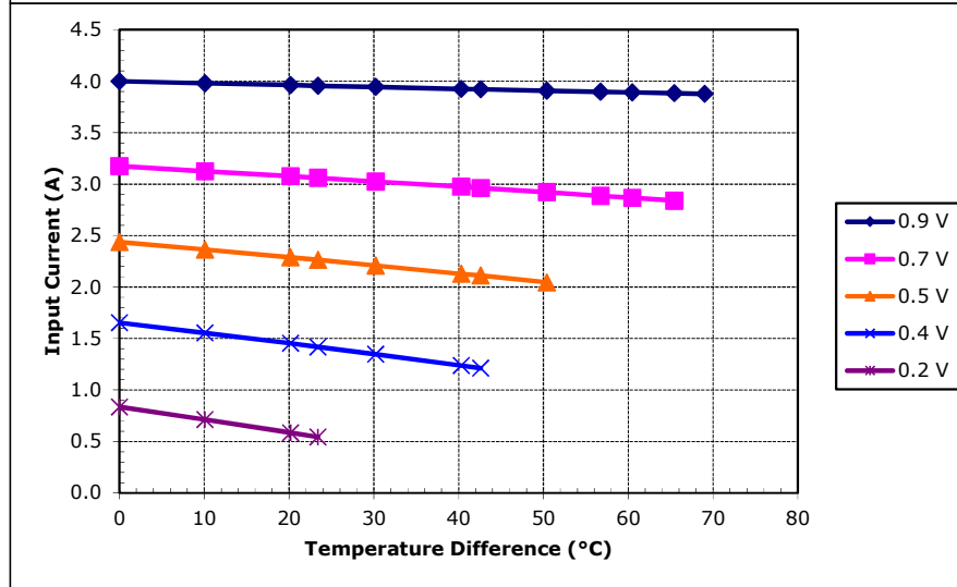
Potted TE-7-1.4-2.5 at a hot-side temperature of 50 °C
