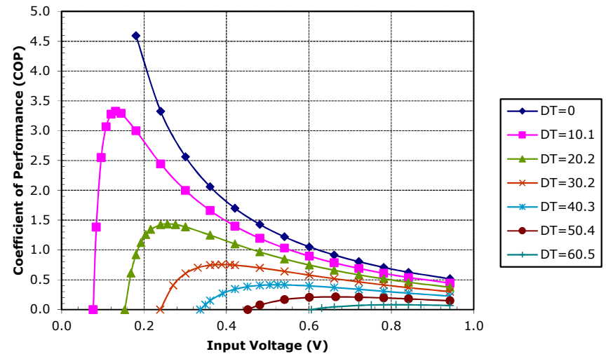
Potted TE-7-1.4-2.5 at a hot-side temperature of 50 °C
