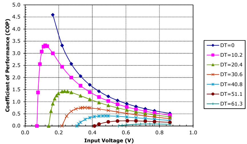
Unpotted TE-7-1.4-2.5 at a hot-side temperature of 30 °C
