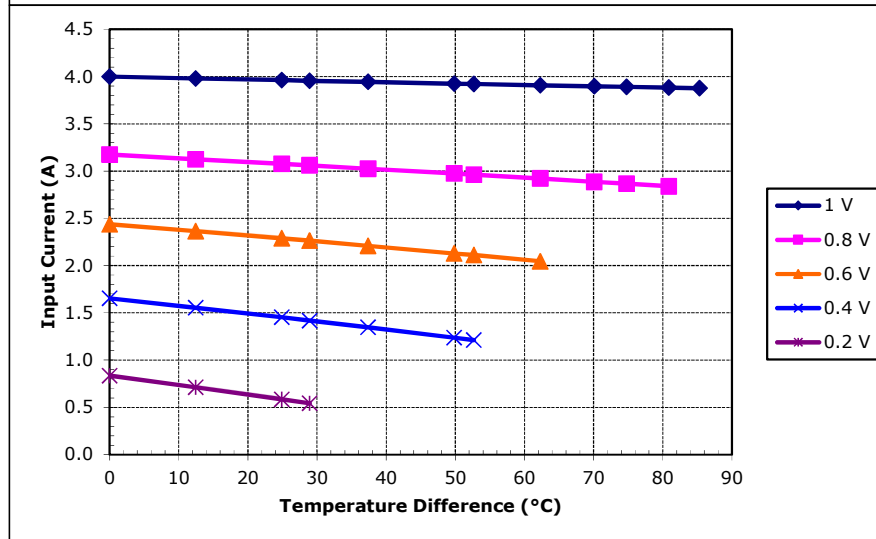
Unpotted TE-7-1.4-2.5 at a hot-side temperature of 70 °C
