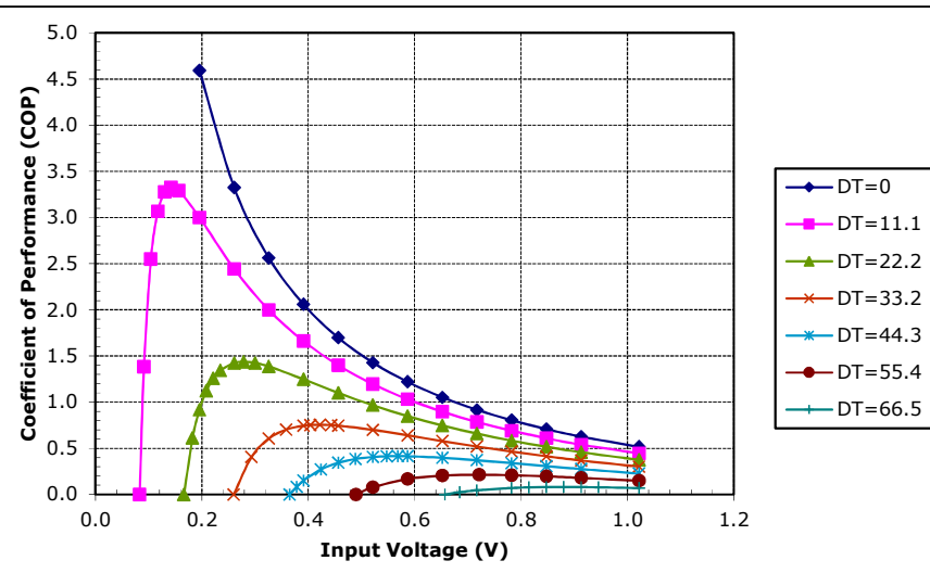
Potted TE-7-1.4-2.5 at a hot-side temperature of 70 °C
