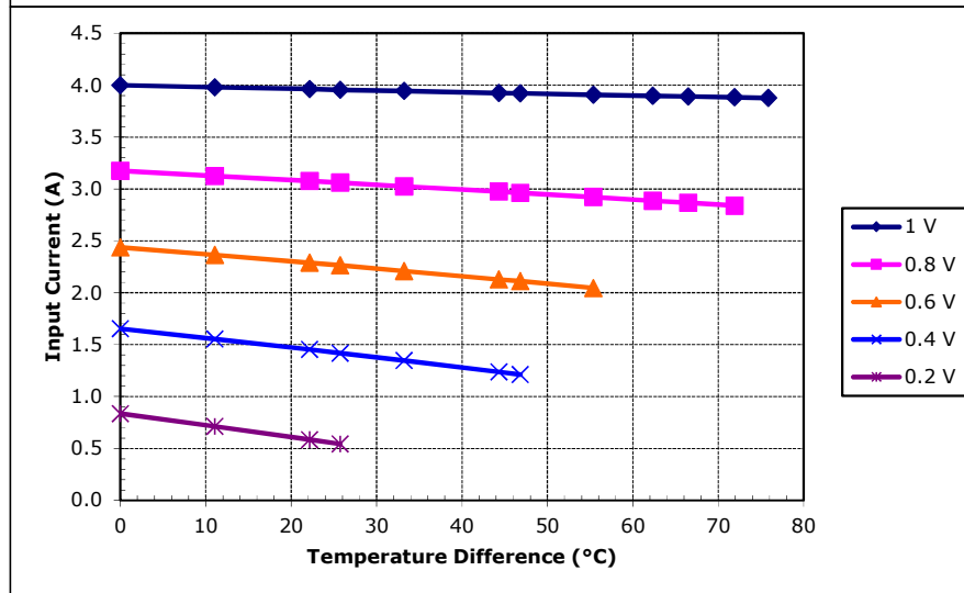
Potted TE-7-1.4-2.5 at a hot-side temperature of 70 °C
