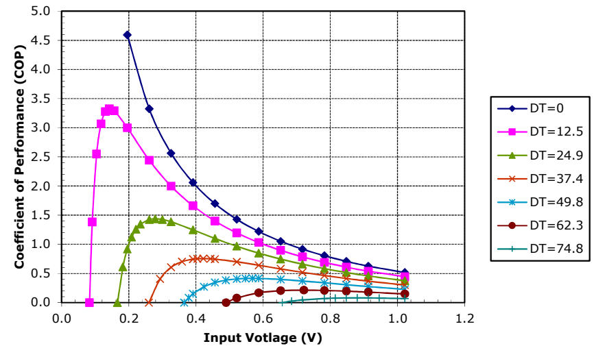
Unpotted TE-7-1.4-2.5 at a hot-side temperature of 70 °C
