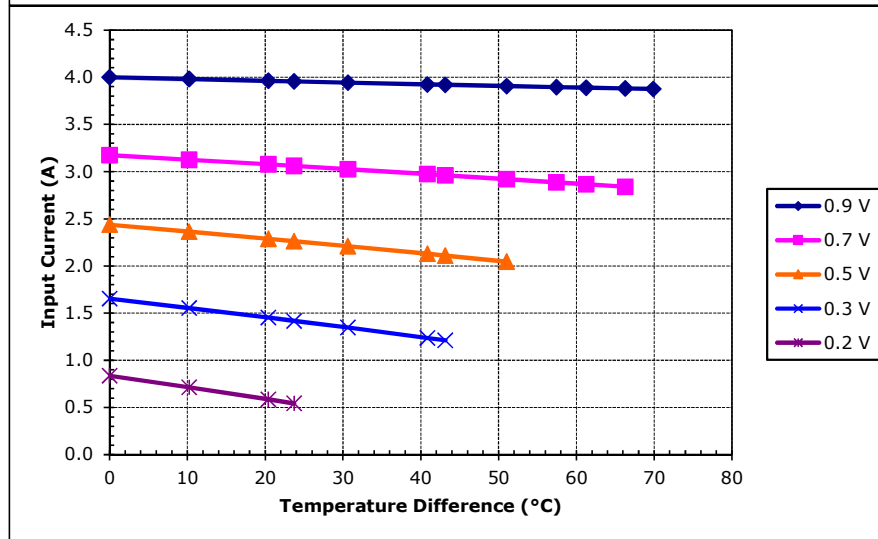
Unpotted TE-7-1.4-2.5 at a hot-side temperature of 30 °C
