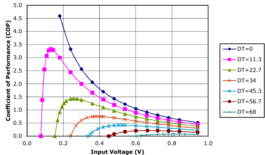
Unpotted TE-7-1.4-2.5 at a hot-side temperature of 50 °C
