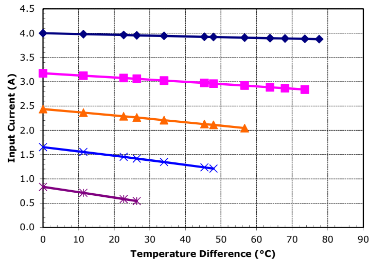
Unpotted TE-7-1.4-2.5 at a hot-side temperature of 50 °C
