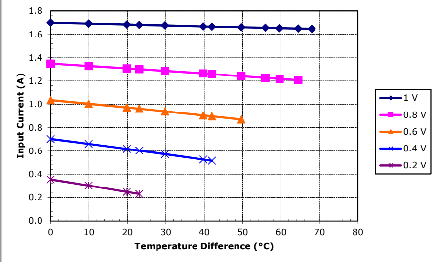
Potted TE-7-0.6-1.0 at a hot-side temperature of 50 °C
