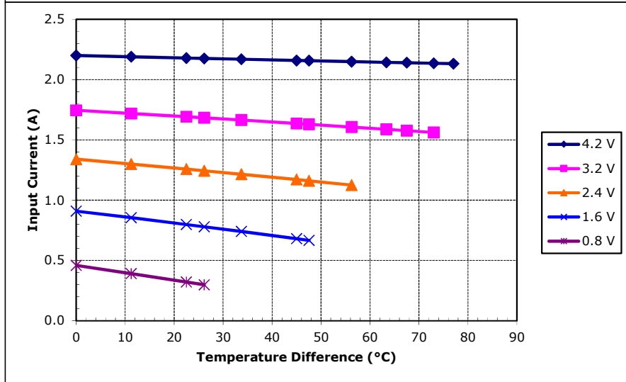
Unpotted TE-31-0.6-0.8 at a hot-side temperature of 50 °C
