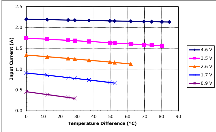
Unpotting TE-31-0.6-0.8 at a hot-side temperature of 70 °C
