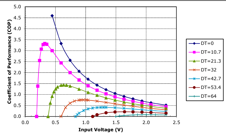
Potted TE-17-0.6-1.5 at a hot-side temperature of 50 °C
