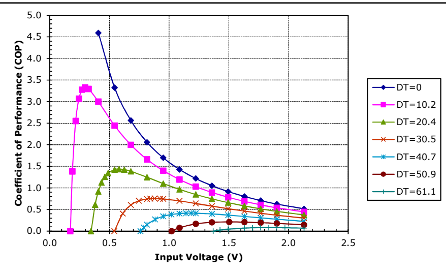
Unpotted TE-17-0.6-1.0 at a hot-side temperature of 30 °C
