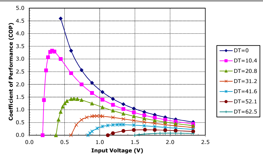
Potted TE-17-0.6-1.0 at a hot-side temperature of 50 °C
