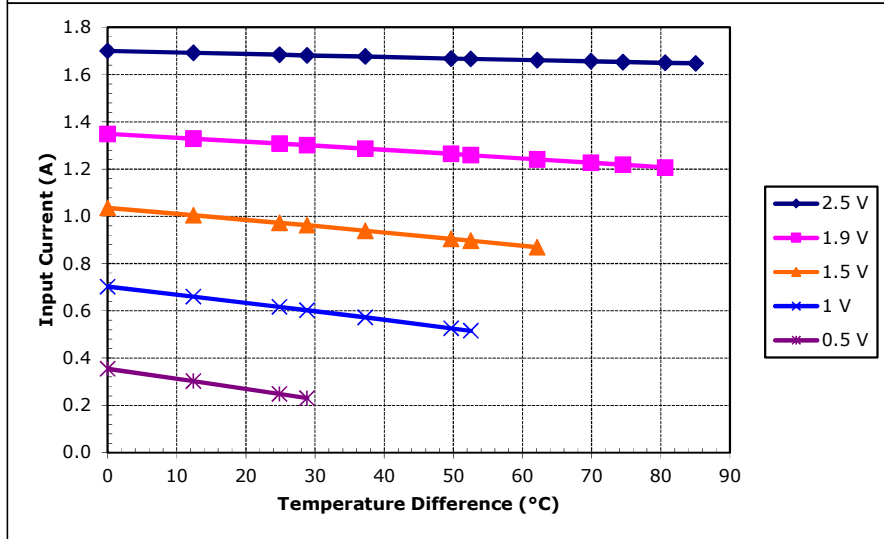
Unpotted TE-17-0.6-1.0 at a hot-side temperature of 70 °C
