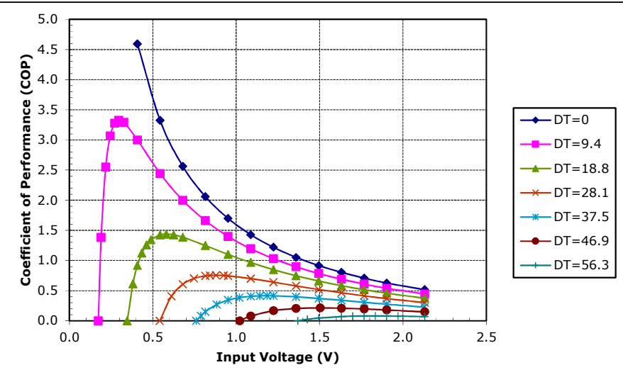
Potted TE-17-0.6-1.0 at a hot-side temperature of 30 °C
