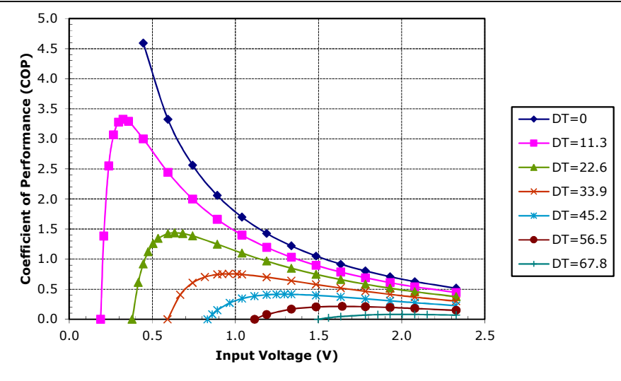
Unpotted TE-17-0.6-1.0 at a hot-side temperature of 50 °C
