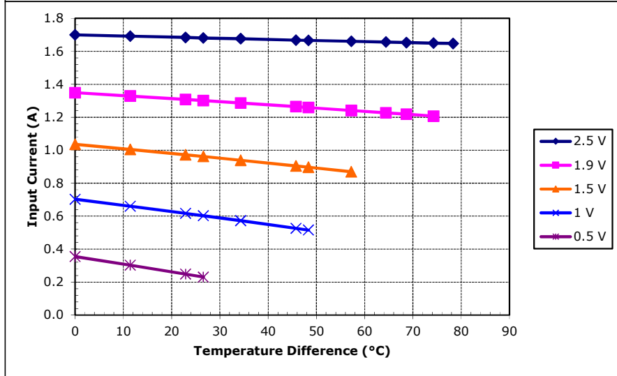
Potted TE-17-0.6-1.0 at a hot-side temperature of 70 °C
