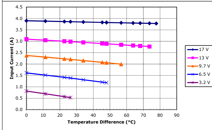
Unpotted TE-127-1.4-2.5 at a hot-side temperature of 50 °C
