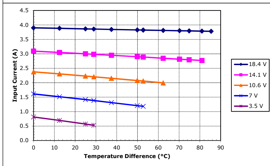
Unpotted TE-127-1.4-2.5 at a hot-side temperature of 70 °C
