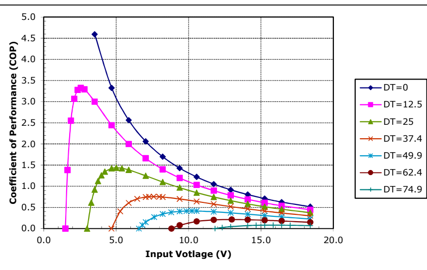
Unpotted TE-127-1.4-2.5 at a hot-side temperature of 70 °C
