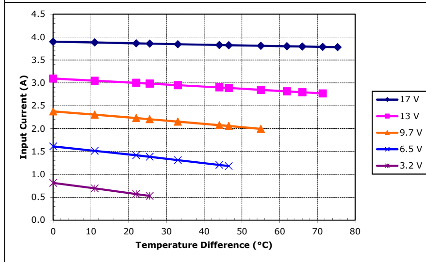
Potted TE-127-1.4-2.5 at a hot-side temperature of 50 °C
