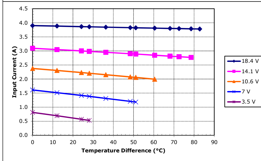
Potted TE-127-1.4-2.5 at a hot-side temperature of 70 °C
