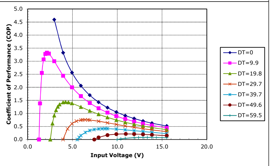
Potted TE-127-1.4-2.5 at a hot-side temperature of 30 °C
