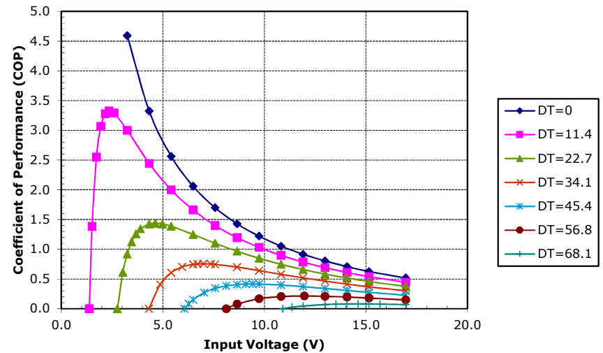
Unpotted TE-127-1.4-2.5 at a hot-side temperature of 50 °C
