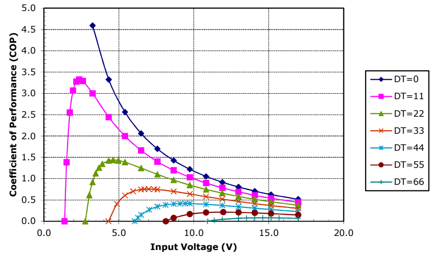
Potted TE-127-1.4-2.5 at a hot-side temperature of 50 °C
