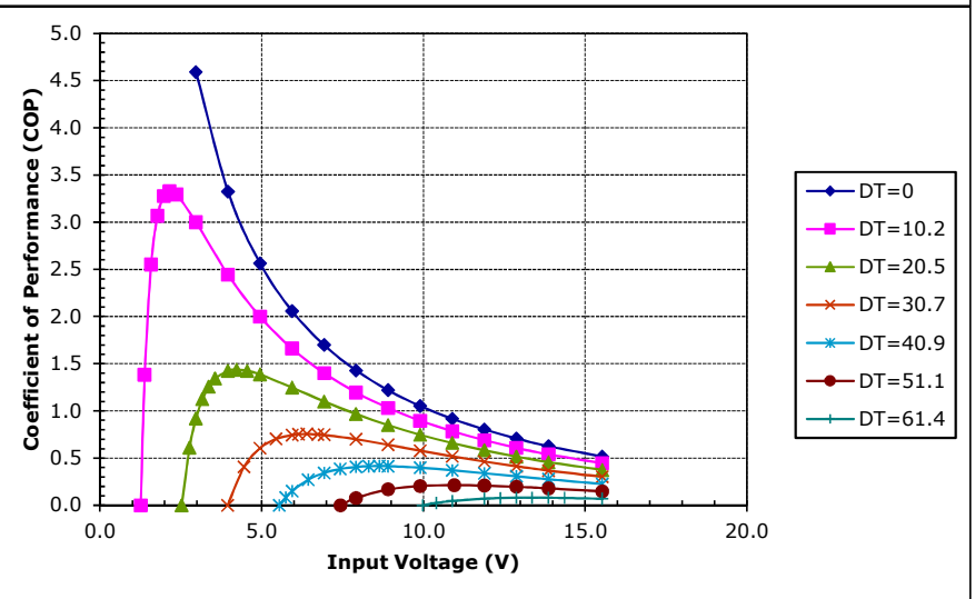
Unpotted TE-127-1.4-2.5 at a hot-side temperature of 30 °C
