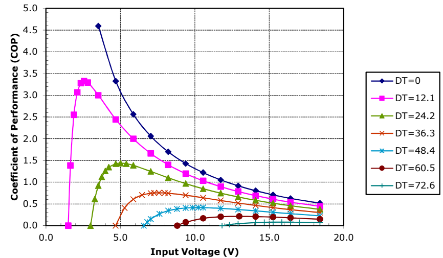
Potted TE-127-1.4-2.5 at a hot-side temperature of 70 °C
