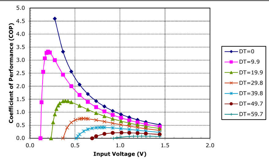
Potted TE-11-0.6-1.5 at a hot-side temperature of 50 °C
