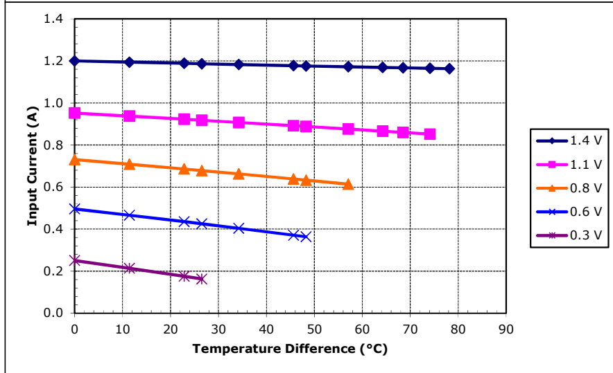
Unpotted TE-11-0.6-1.5 at a hot-side temperature of 50 °C
