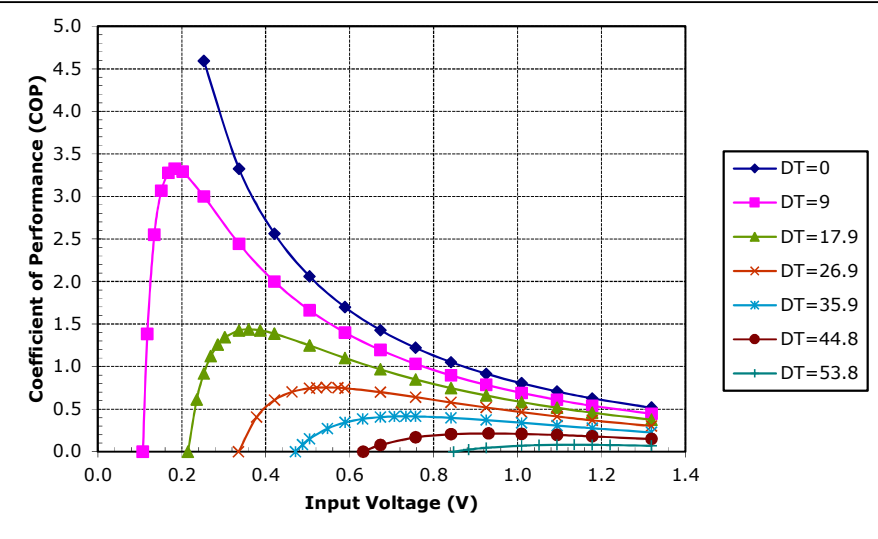
Potted TE-11-0.6-1.5 at a hot-side temperature of 30 °C
