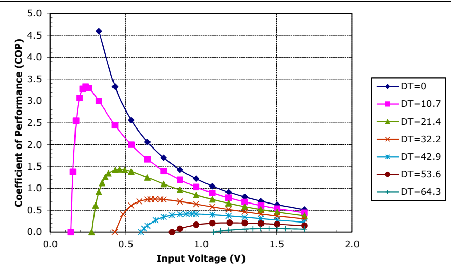
Potted TE-11-0.6-1.2 at a hot-side temperature of 70 °C
