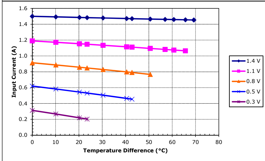
Unpotted TE-11-0.6-1.2 at a hot-side temperature of 30 °C
