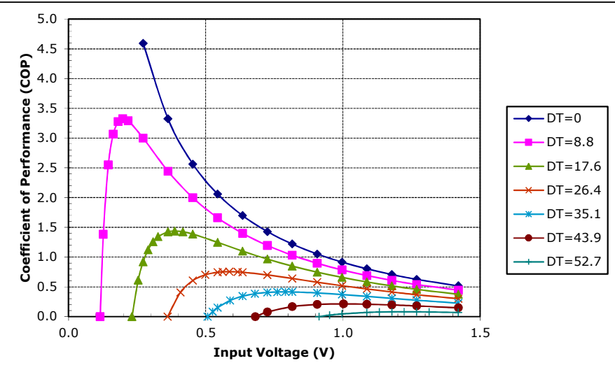
Potted TE-11-0.6-1.2 at a hot-side temperature of 30 °C
