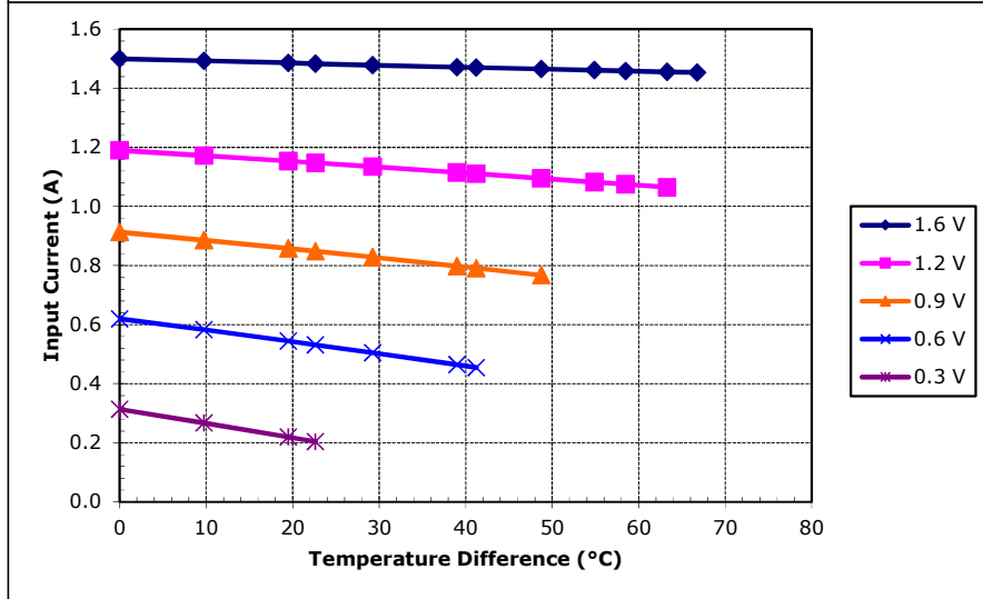
Potted TE-11-0.6-1.2 at a hot-side temperature of 50 °C
