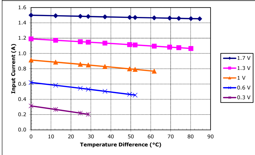
Unpotted TE-11-0.6-1.2 at a hot-side temperature of 70 °C
