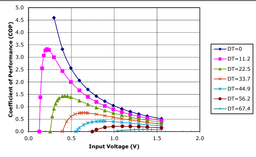
Unpotted TE-11-0.6-1.2 at a hot-side temperature of 50 °C
