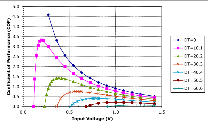
Unpotted TE-11-0.6-1.0 at a hot-side temperature of 30 °C
