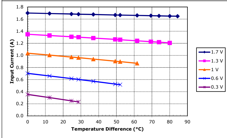
Unpotted TE-11-0.6-1.0 at a hot-side temperature of 70 °C
