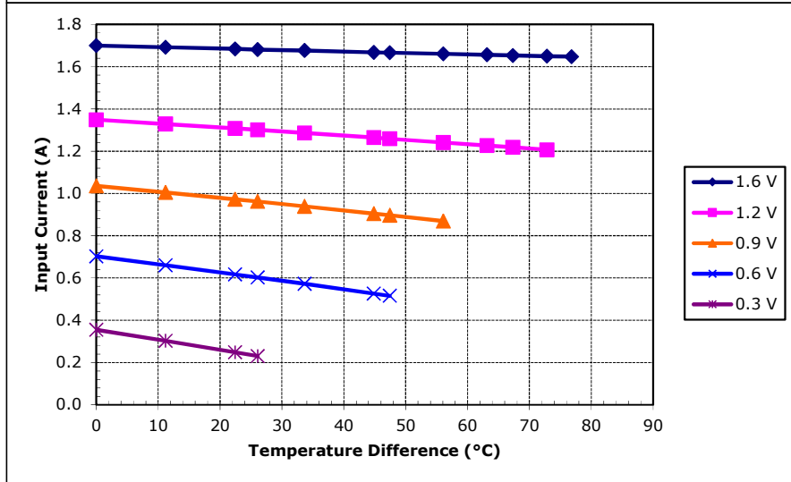
Unpotted TE-11-0.6-1.0 at a hot-side temperature of 50 °C
