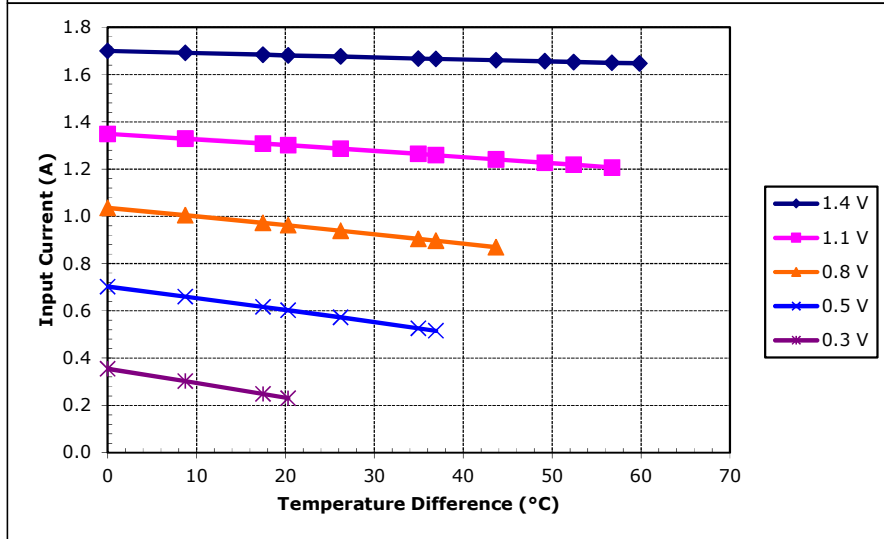
Potted TE-11-0.6-1.0 at a hot-side temperature of 30 °C
