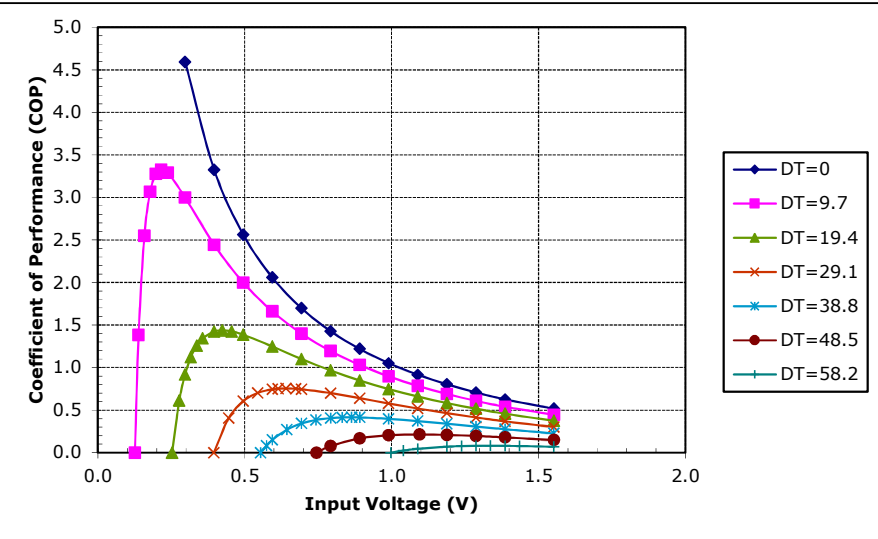
Potted TE-11-0.6-1.0 at a hot-side temperature of 50 °C
