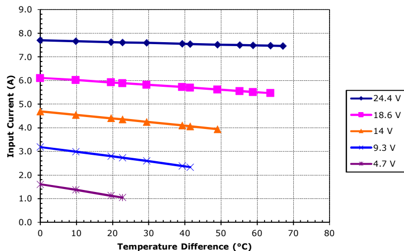
Unpotted HP-199-1.4-1.15 at a hot-side temperature of 30 °C
