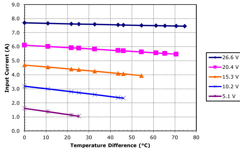
Unpotted HP-199-1.4-1.15 at a hot-side temperature of 50 °C
