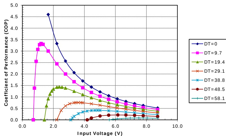
Potted TE-71-1.0-2.0 at a hot-side temperature of 30 °C
