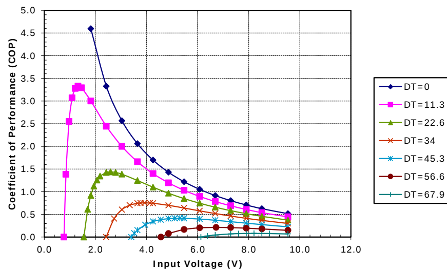
Unpotted TE-71-1.0-2.0 at a hot-side temperature of 50 °C
