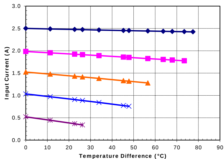
Unpotted TE-71-1.0-2.0 at a hot-side temperature of 50 °C
