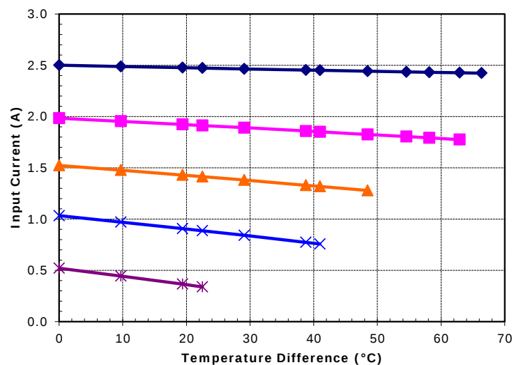
Potted TE-71-1.0-2.0 at a hot-side temperature of 30 °C
