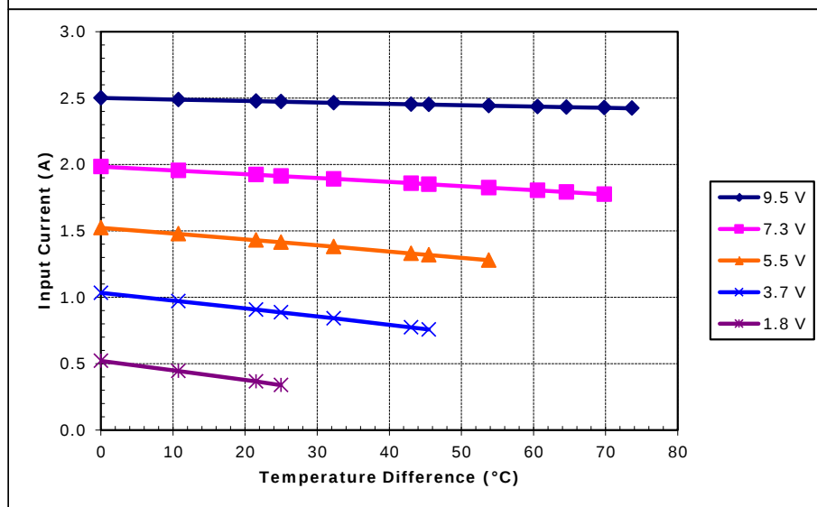
Potted TE-71-1.0-2.0 at a hot-side temperature of 50 °C
