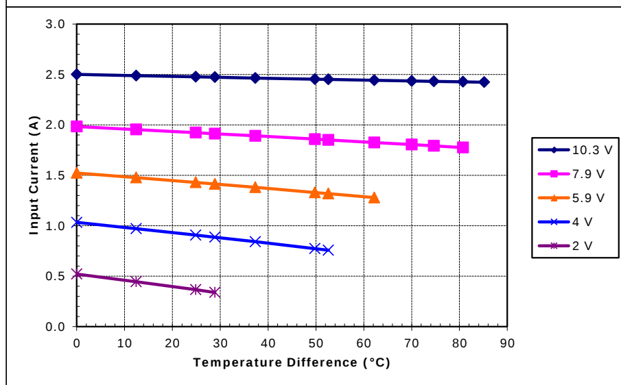
Unpotted TE-71-1.0-2.0 at a hot-side temperature of 70 °C
