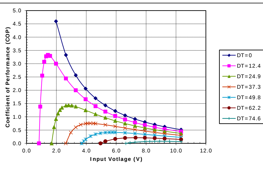
Unpotted TE-71-1.0-2.0 at a hot-side temperature of 70 °C
