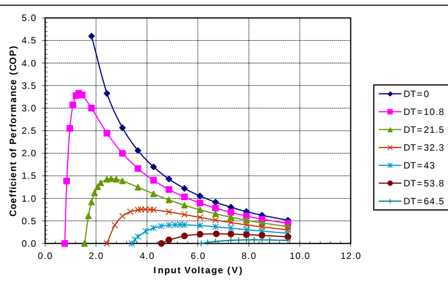
Potted TE-71-1.0-2.0 at a hot-side temperature of 50 °C
