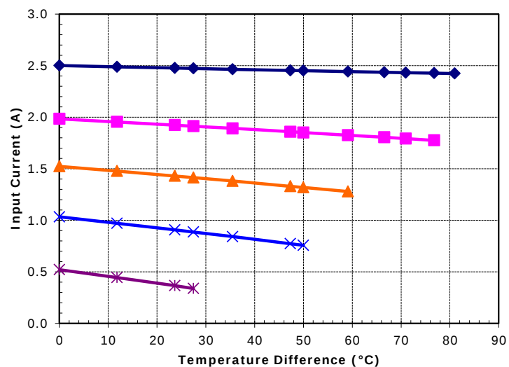
Potted TE-71-1.0-2.0 at a hot-side temperature of 70 °C
