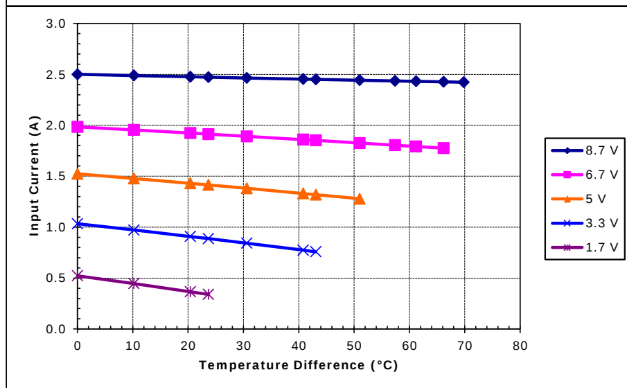
Unpotted TE-71-1.0-2.0 at a hot-side temperature of 30 °C
