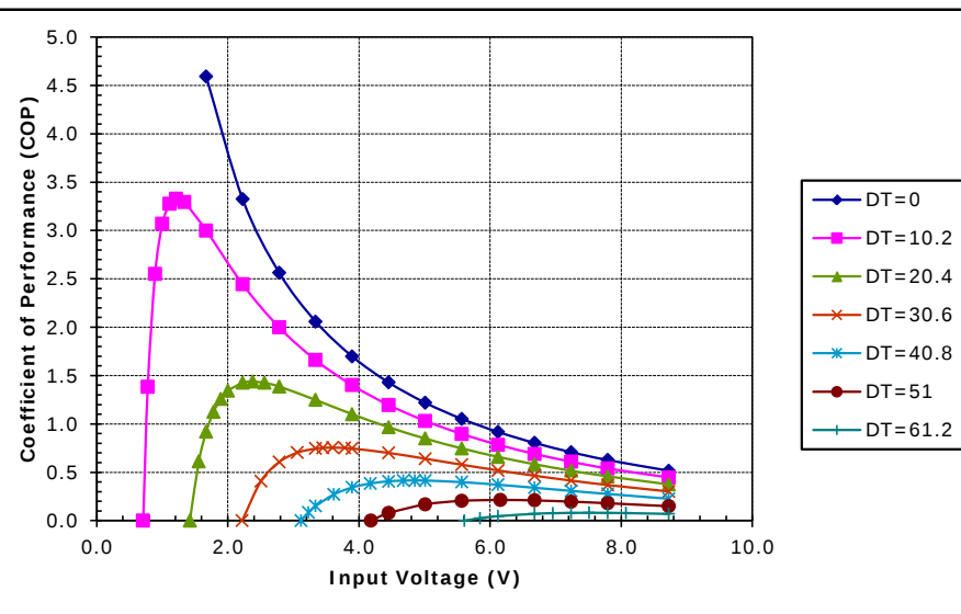
Unpotted TE-71-1.0-2.0 at a hot-side temperature of 30 °C
