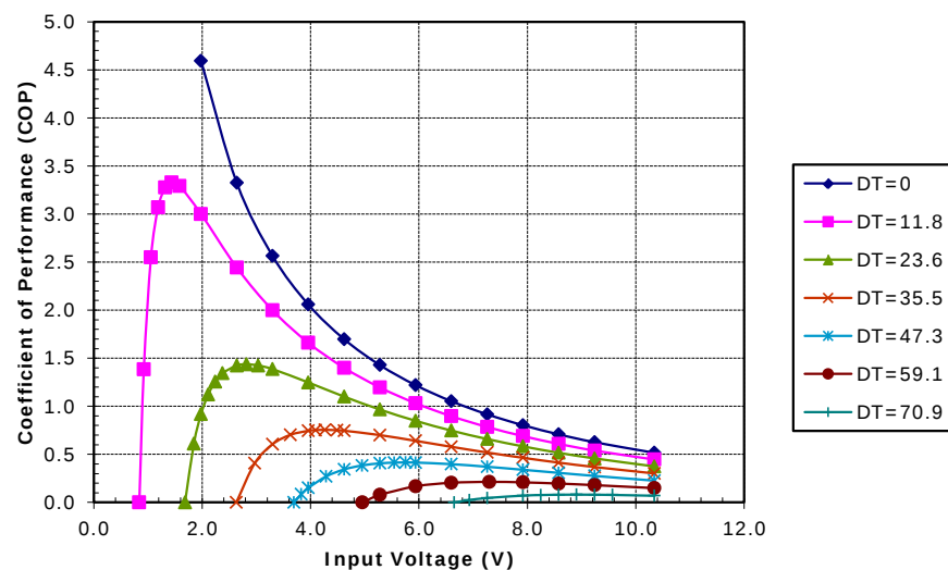
Potted TE-71-1.0-2.0 at a hot-side temperature of 70 °C
