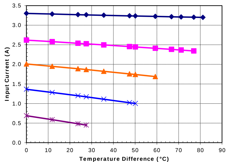
Potted TE-71-1.0-1.5 at a hot-side temperature of 70 °C
