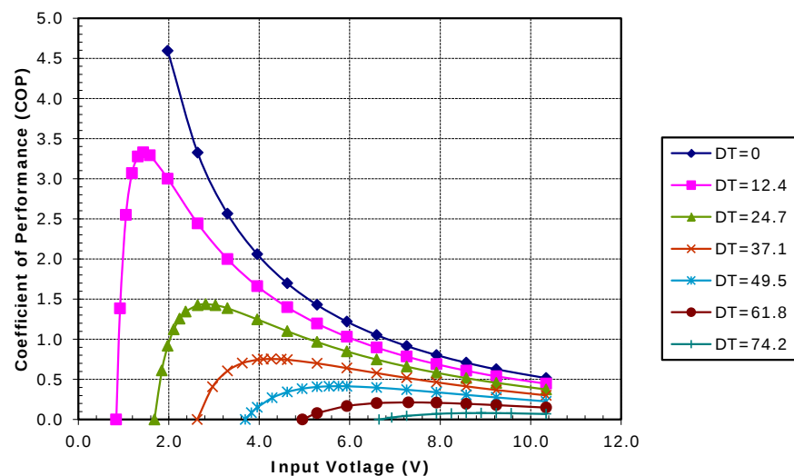
Unpotted TE-71-1.0-1.5 at a hot-side temperature of 70 °C
