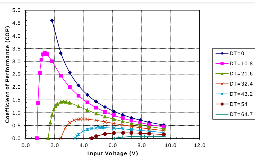
Potted TE-71-1.0-1.5 at a hot-side temperature of 50 °C
