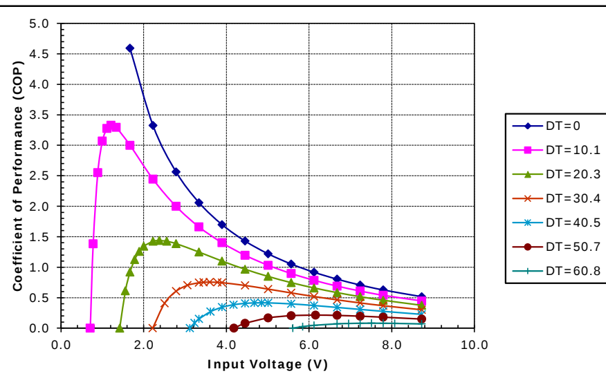
Unpotted TE-71-1.0-1.5 at a hot-side temperature of 30 °C
