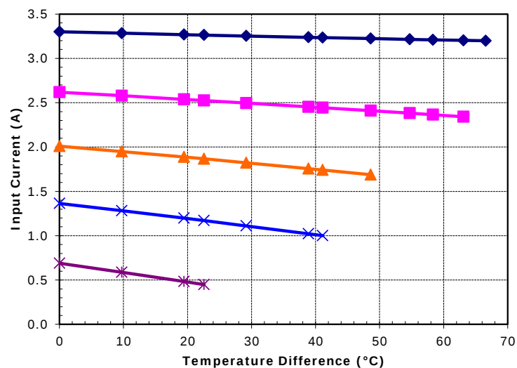
Potted TE-71-1.0-1.5 at a hot-side temperature of 30 °C
