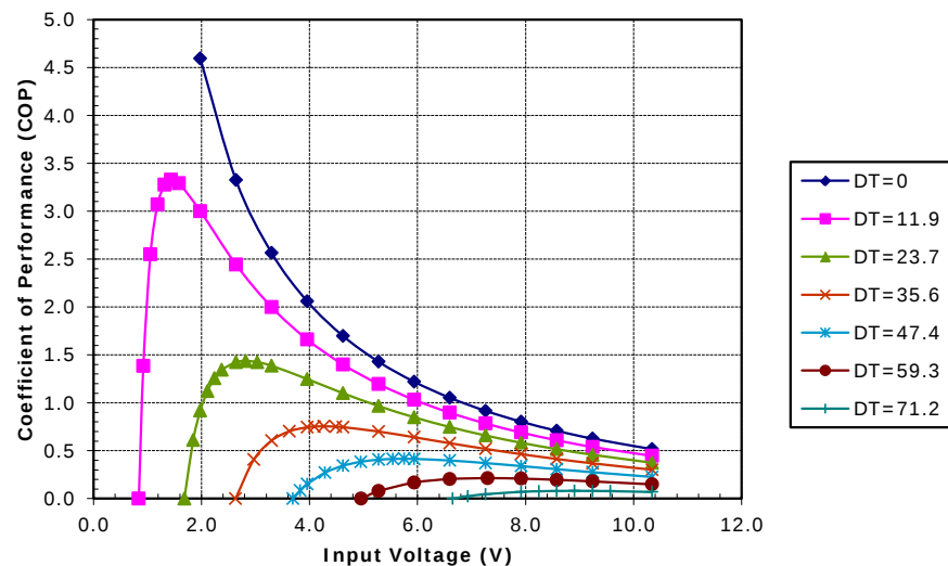
Potted TE-71-1.0-1.5 at a hot-side temperature of 70 °C
