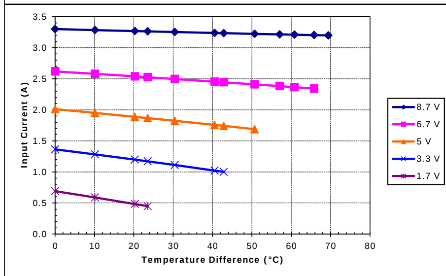
Unpotted TE-71-1.0-1.5 at a hot-side temperature of 30 °C
