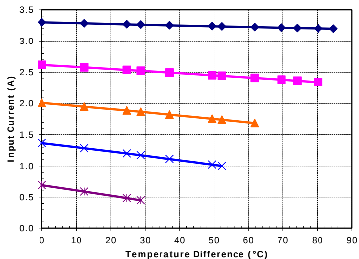
Unpotted TE-71-1.0-1.5 at a hot-side temperature of 70 °C
