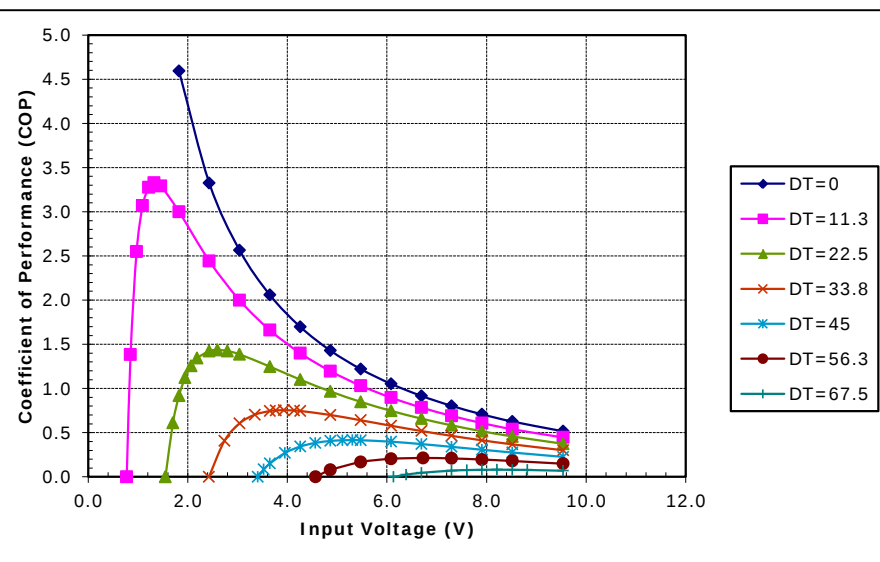
Unpotted TE-71-1.0-1.5 at a hot-side temperature of 50 °C
