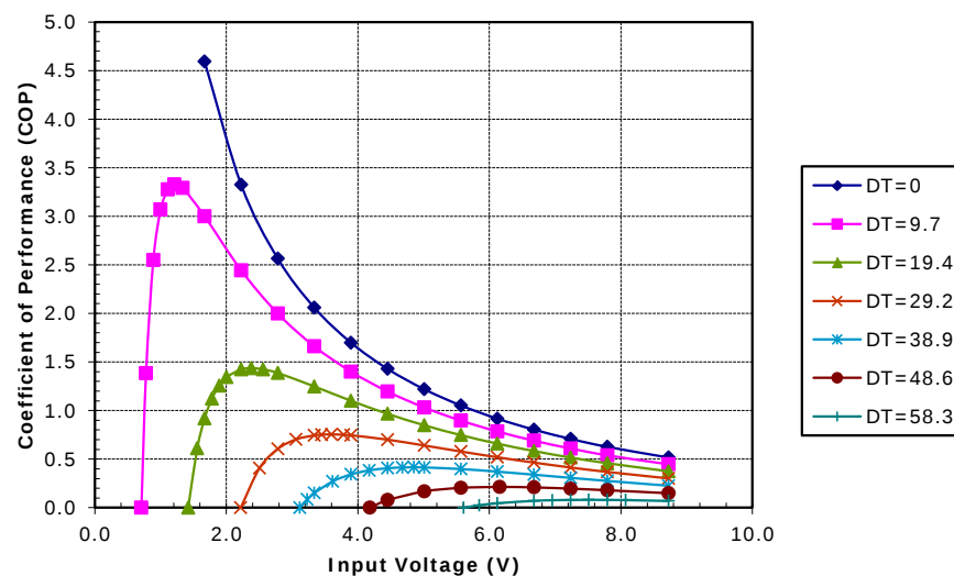
Potted TE-71-1.0-1.5 at a hot-side temperature of 30 °C
