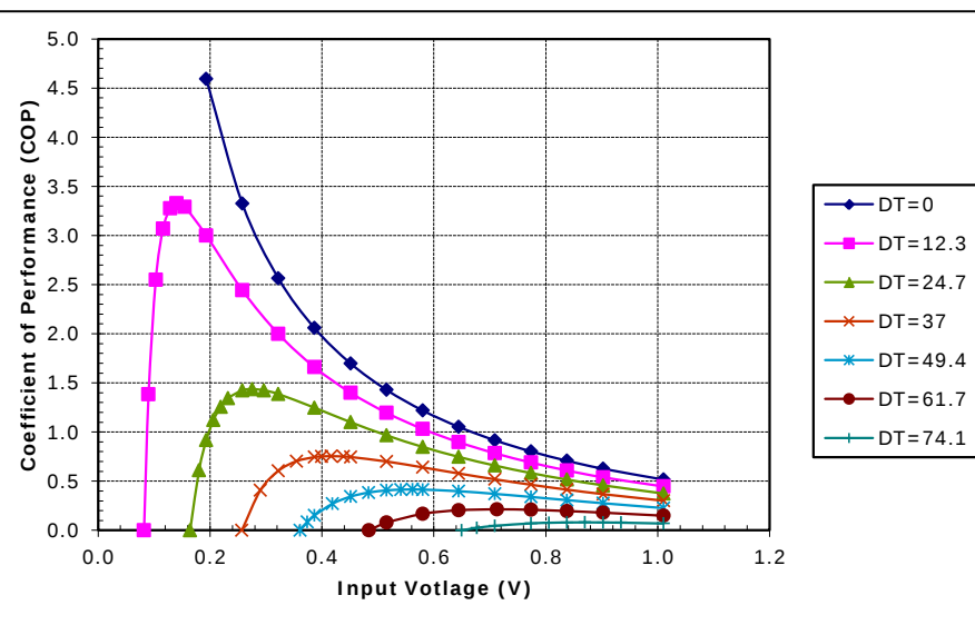
Unpotted TE-7-1.0-2.0 at a hot-side temperature of 70 °C
