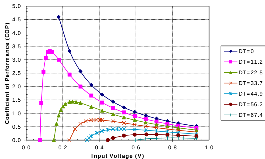
Unpotted TE-7-1.0-2.0 at a hot-side temperature of 50 °C
