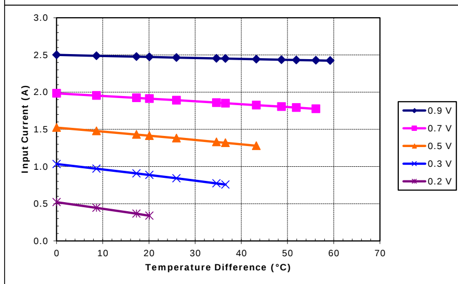
Potted TE-7-1.0-2.0 at a hot-side temperature of 30 °C
