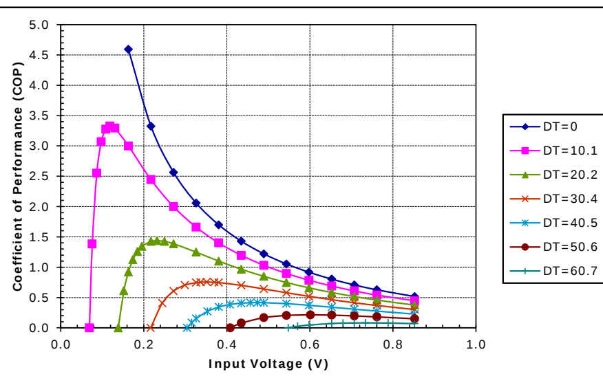
Unpotted TE-7-1.0-2.0 at a hot-side temperature of 30 °C
