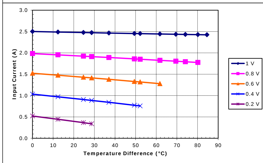
Unpotted TE-7-1.0-2.0 at a hot-side temperature of 70 °C
