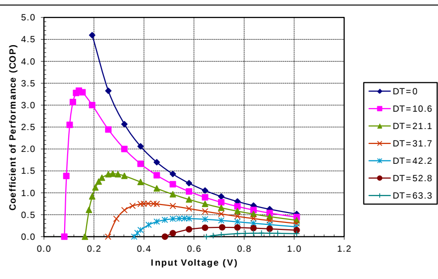
Potted TE-7-1.0-2.0 at a hot-side temperature of 70 °C
