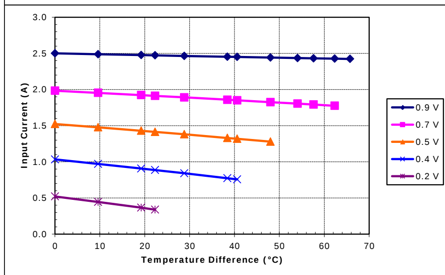
Potted TE-7-1.0-2.0 at a hot-side temperature of 50 °C
