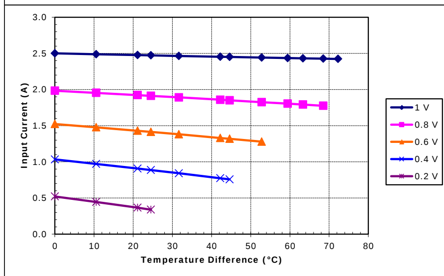
Potted TE-7-1.0-2.0 at a hot-side temperature of 70 °C
