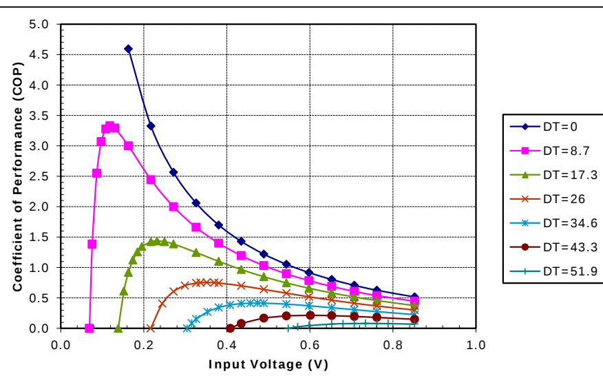
Potted TE-7-1.0-2.0 at a hot-side temperature of 30 °C
