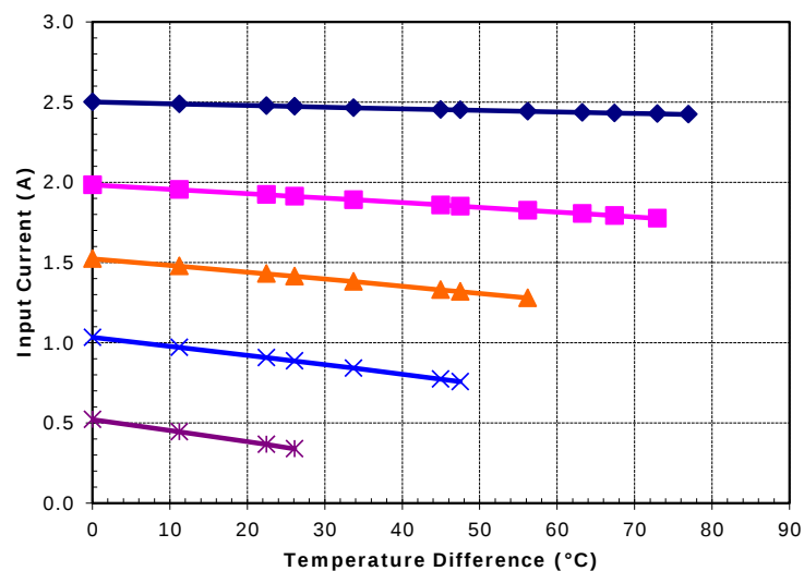
Unpotted TE-7-1.0-2.0 at a hot-side temperature of 50 °C
