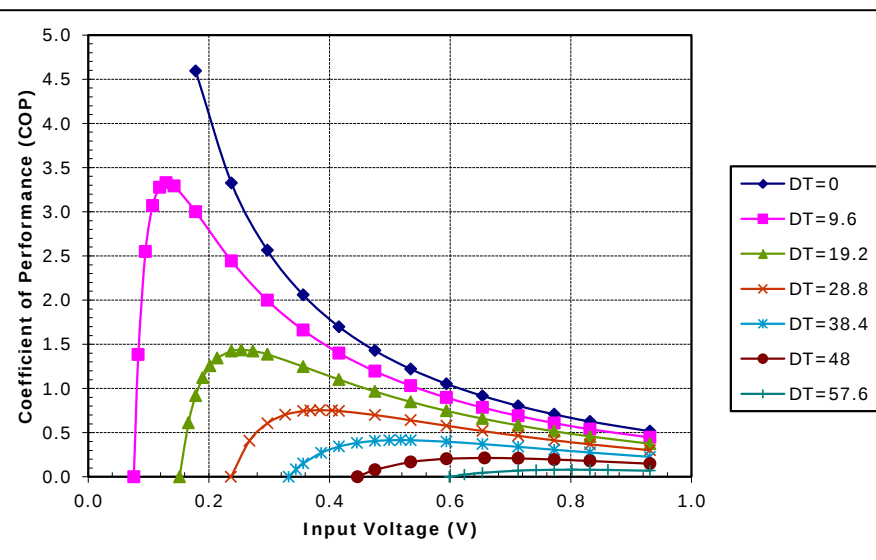
Potted TE-7-1.0-2.0 at a hot-side temperature of 50 °C
