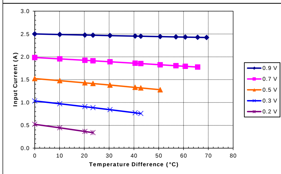
Unpotted TE-7-1.0-2.0 at a hot-side temperature of 30 °C
