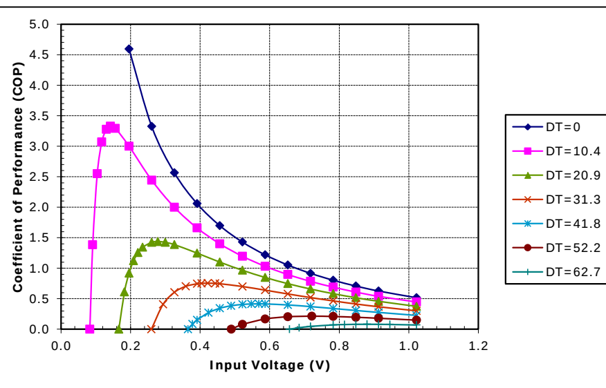
Potted TE-7-1.0-1.5 at a hot-side temperature of 70 °C
