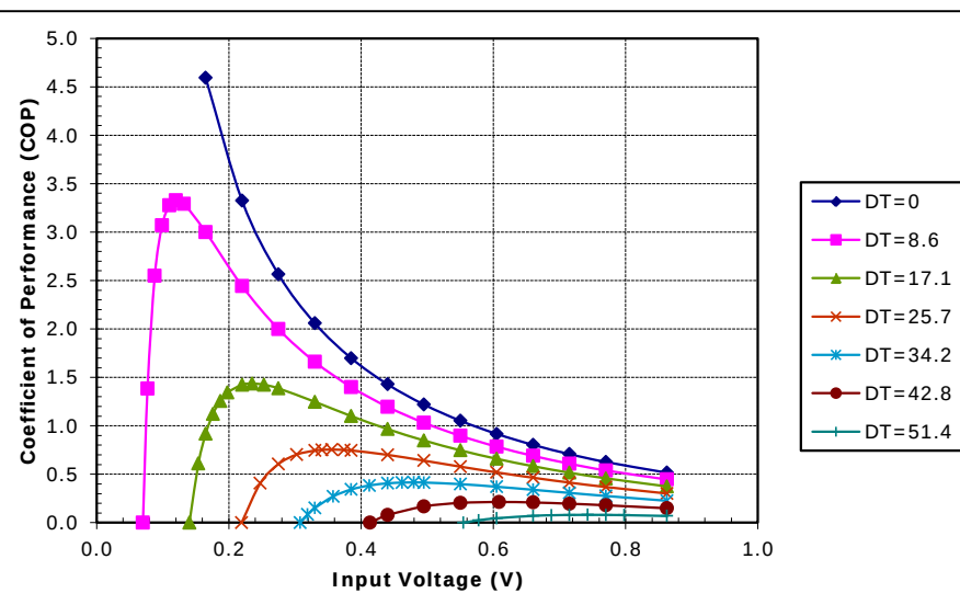
Potted TE-7-1.0-1.5 at a hot-side temperature of 30 °C
