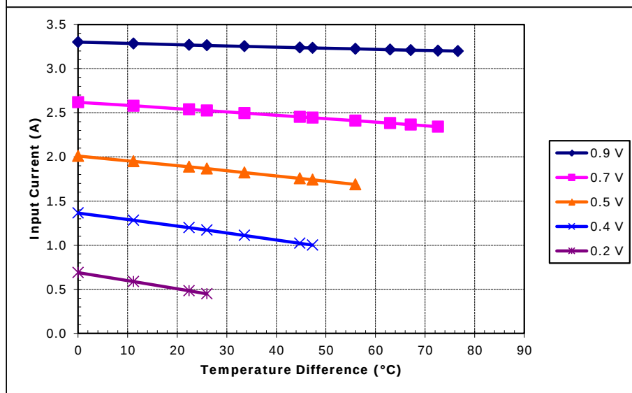
Unpotted TE-7-1.0-1.5 at a hot-side temperature of 50 °C
