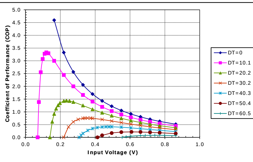
Unpotted TE-7-1.0-1.5 at a hot-side temperature of 30 °C
