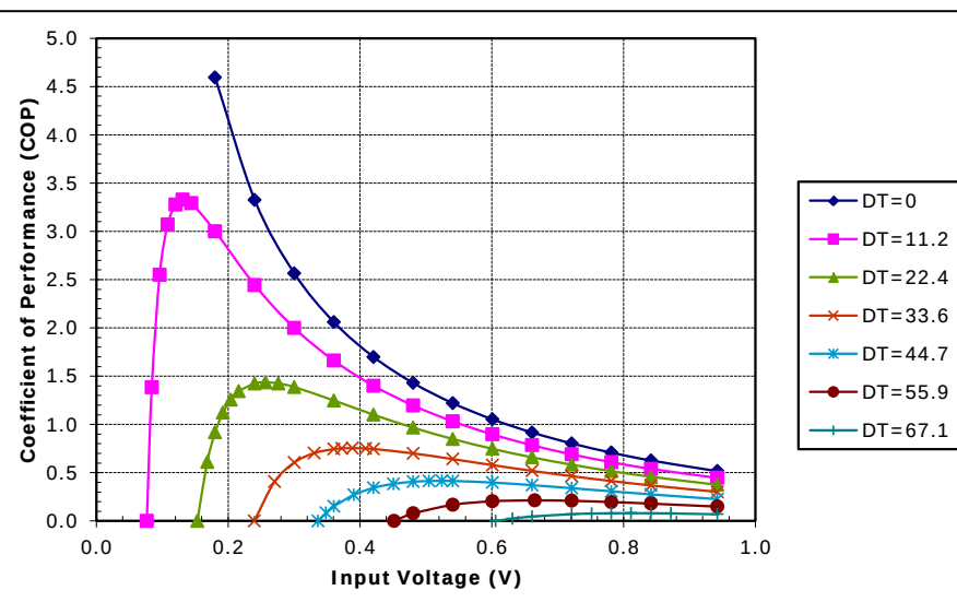
Unpotted TE-7-1.0-1.5 at a hot-side temperature of 50 °C
