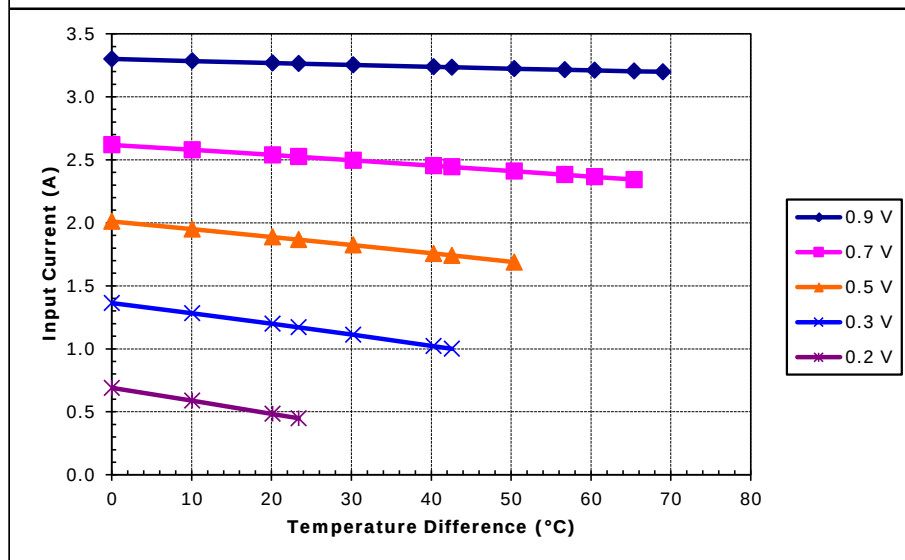
Unpotted TE-7-1.0-1.5 at a hot-side temperature of 30 °C
