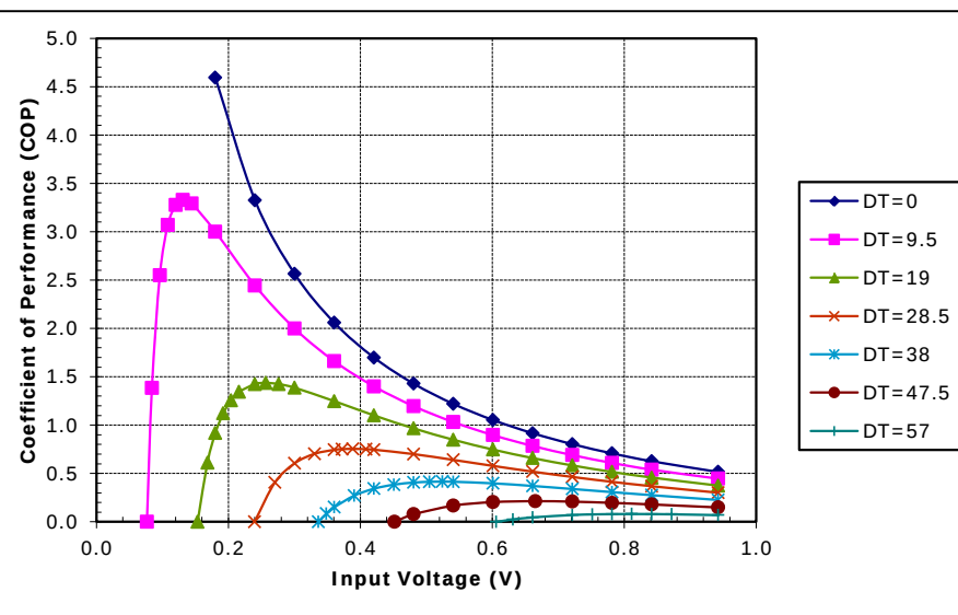
Potted TE-7-1.0-1.5 at a hot-side temperature of 50 °C
