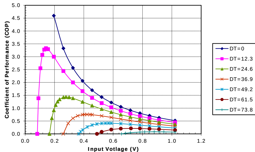
Unpotted TE-7-1.0-1.5 at a hot-side temperature of 70 °C
