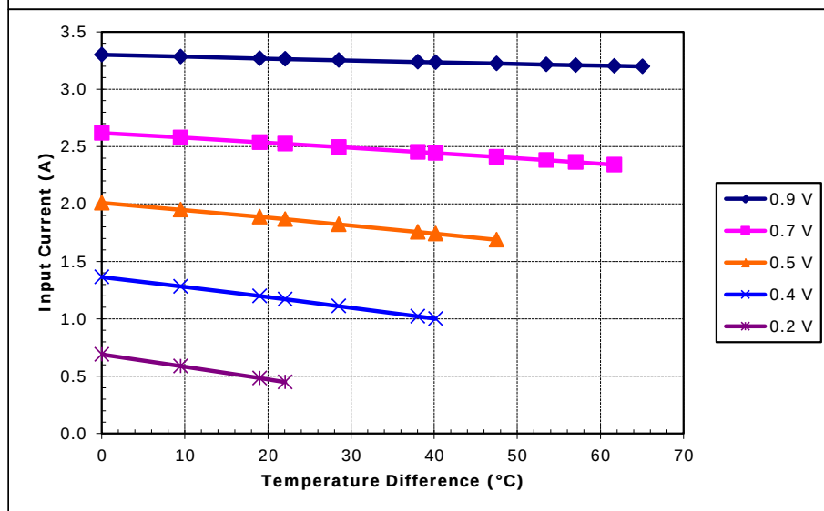
Potted TE-7-1.0-1.5 at a hot-side temperature of 50 °C
