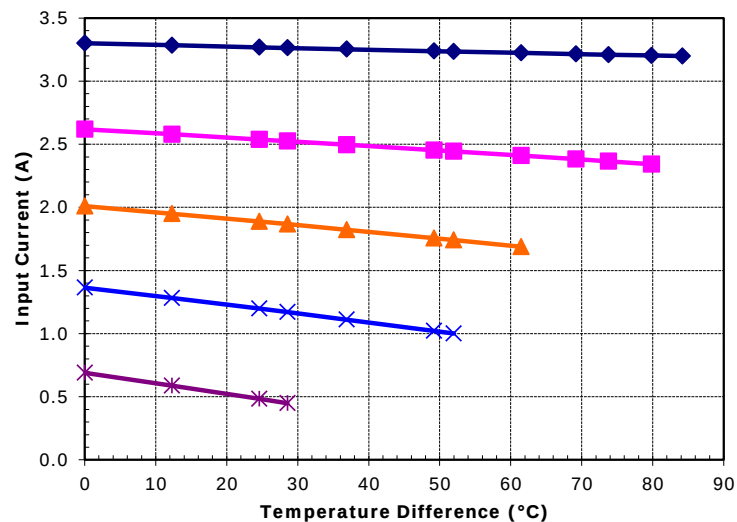
Unpotted TE-7-1.0-1.5 at a hot-side temperature of 70 °C
