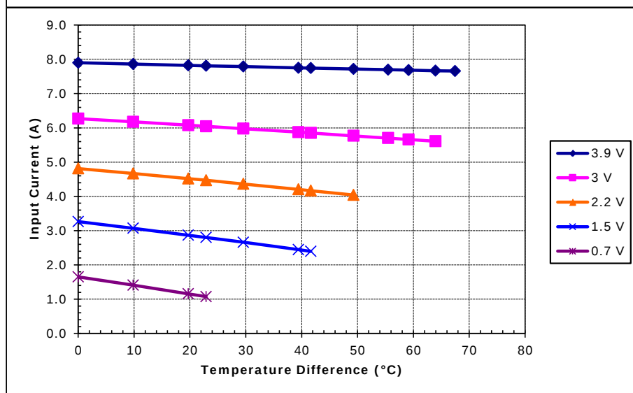
Unpotted TE-31-1.4-1.15 at a hot-side temperature of 30 °C
