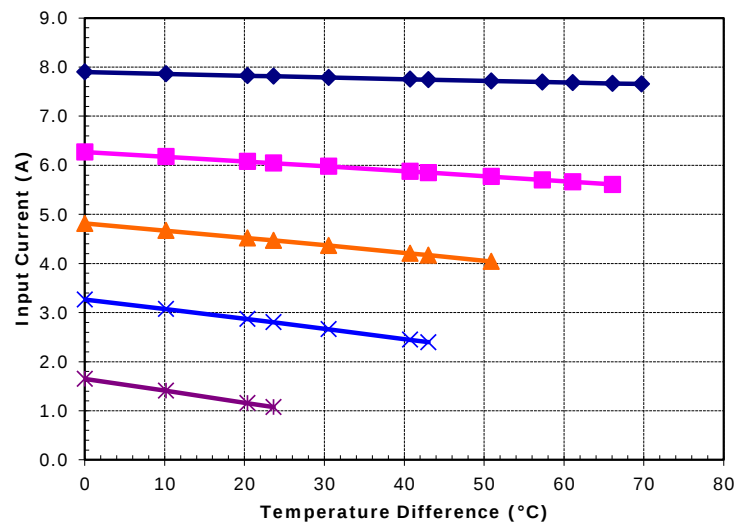
Potted TE-31-1.4-1.15 at a hot-side temperature of 50 °C
