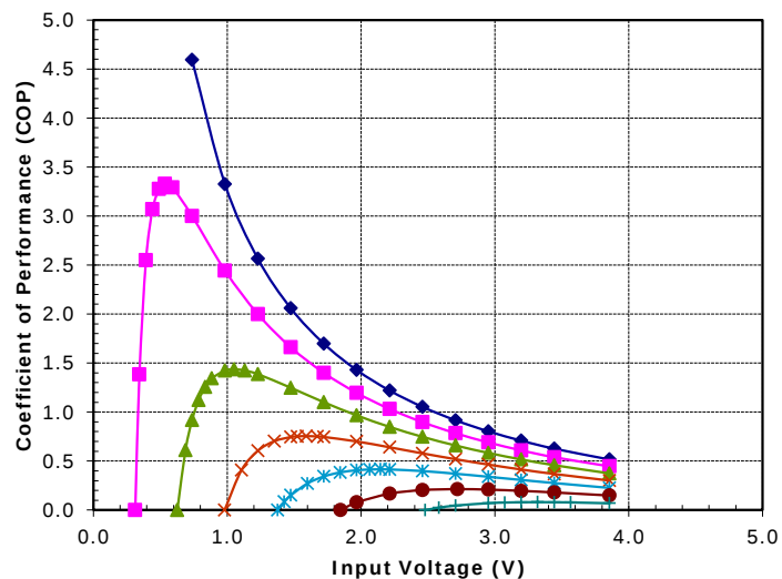
Potted TE-31-1.4-1.15 at a hot-side temperature of 30 °C
