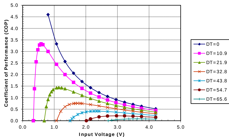
Unpotted TE-31-1.4-1.15 at a hot-side temperature of 50 °C
