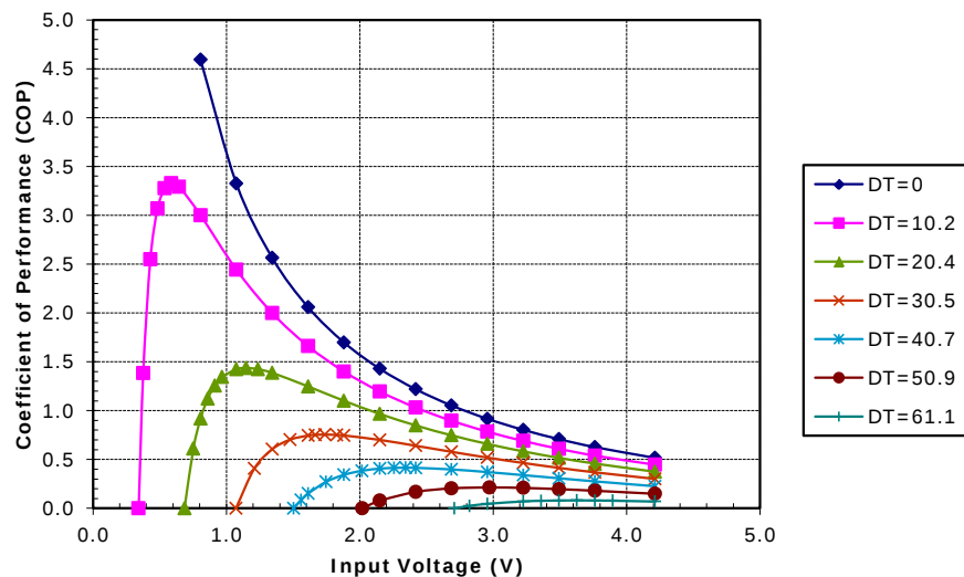
Potted TE-31-1.4-1.15 at a hot-side temperature of 50 °C
