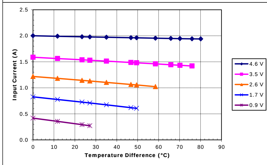
Potted TE-31-1.0-2.5 at a hot-side temperature of 70 °C
