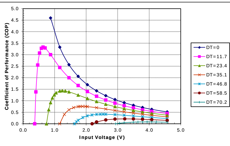
Potted TE-31-1.0-2.5 at a hot-side temperature of 70 °C
