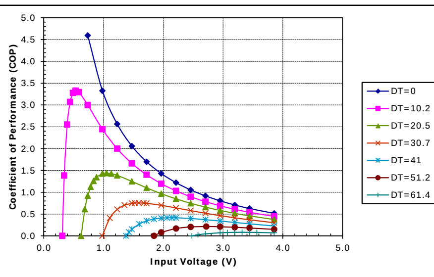
Unpotted TE-31-1.0-2.5 at a hot-side temperature of 30 °C
