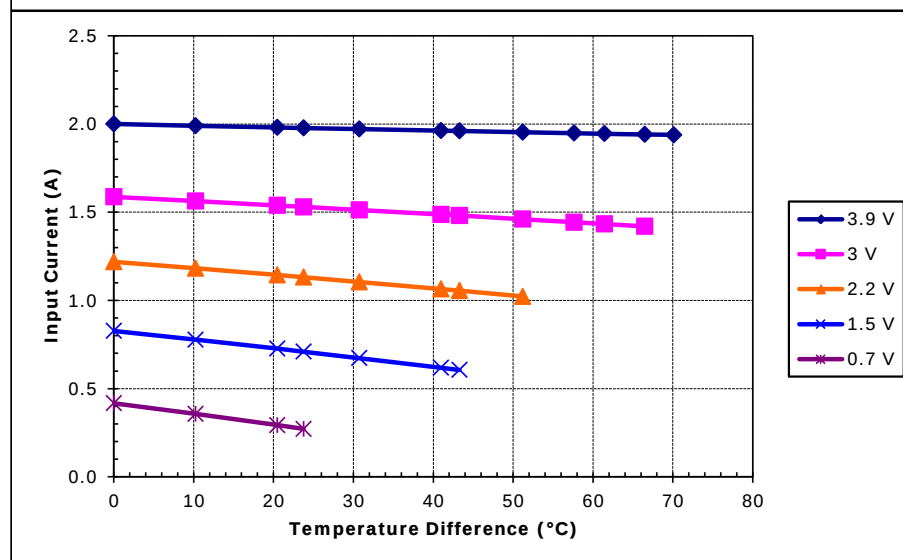
Unpotted TE-31-1.0-2.5 at a hot-side temperature of 30 °C
