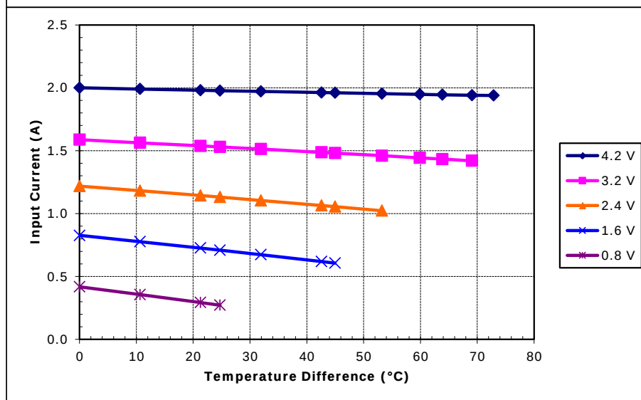
Potted TE-31-1.0-2.5 at a hot-side temperature of 50 °C
