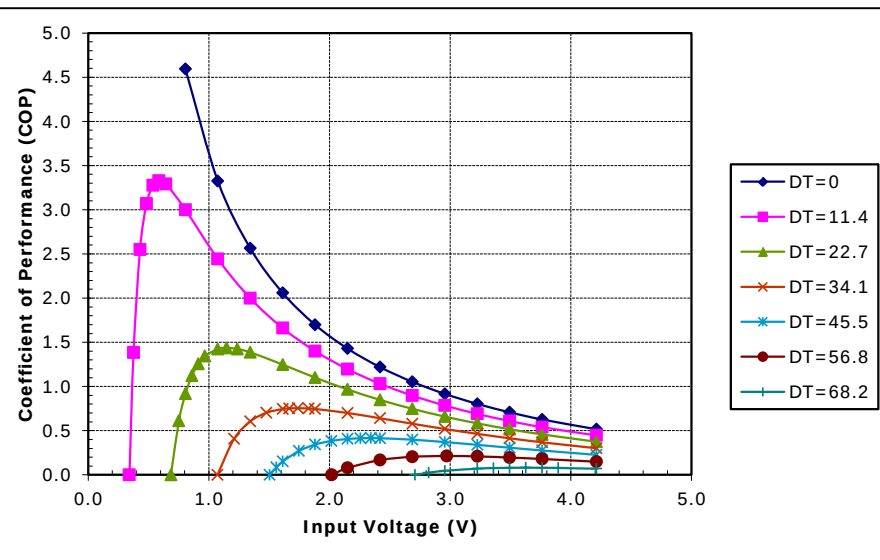
Unpotted TE-31-1.0-2.5 at a hot-side temperature of 50 °C
