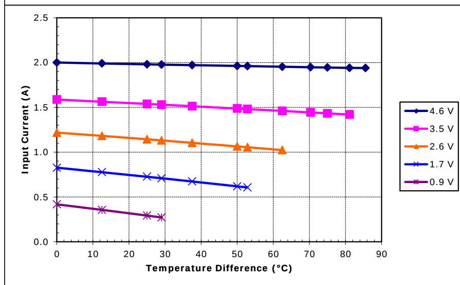
Unpotted TE-31-1.0-2.5 at a hot-side temperature of 70 °C
