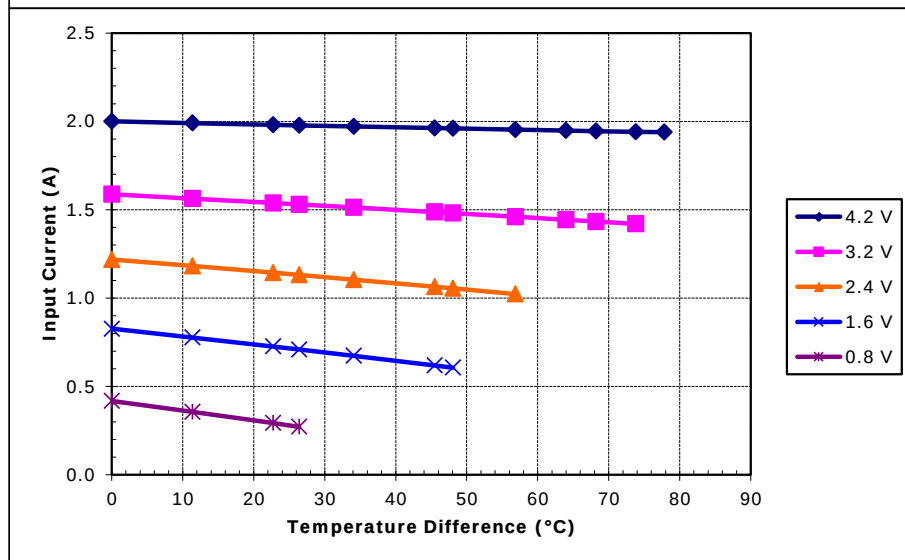
Unpotted TE-31-1.0-2.5 at a hot-side temperature of 50 °C
