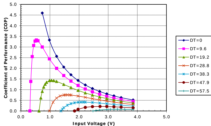
Potted TE-31-1.0-2.5 at a hot-side temperature of 30 °C
