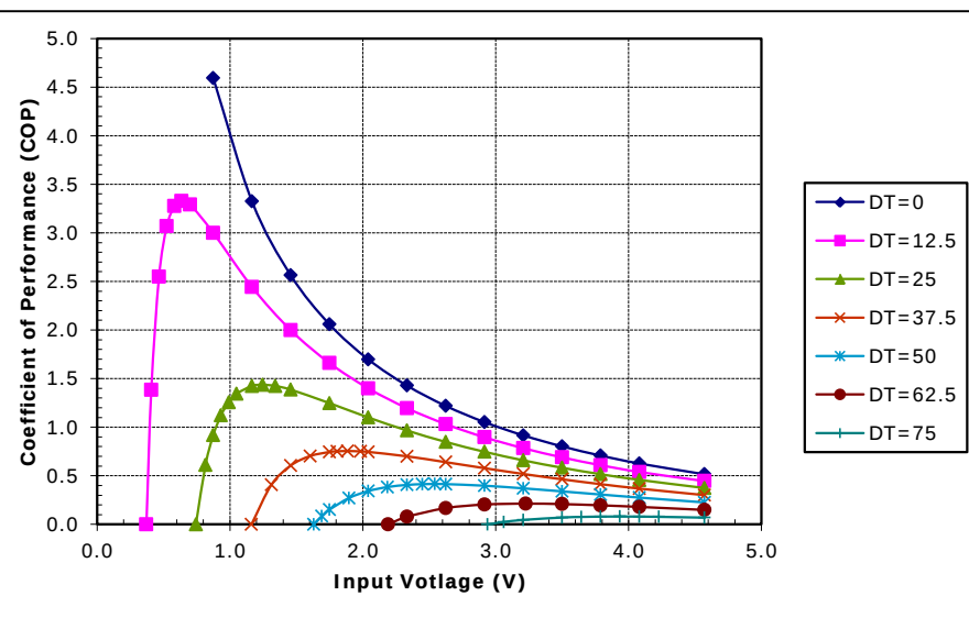
Unpotted TE-31-1.0-2.5 at a hot-side temperature of 70 °C
