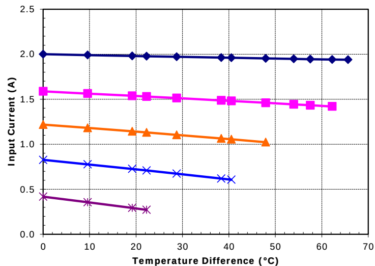
Potted TE-31-1.0-2.5 at a hot-side temperature of 30 °C
