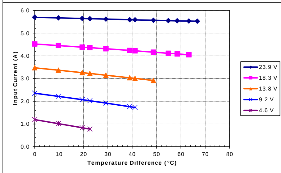
Unpotted TE-195-1.0-0.8 at a hot-side temperature of 30 °C
