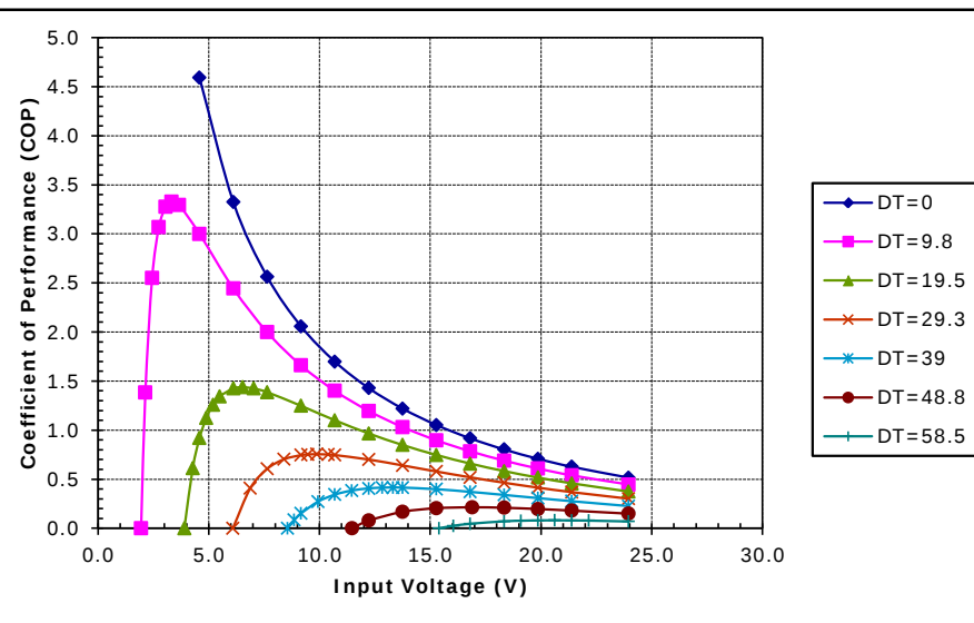
Unpotted TE-195-1.0-0.8 at a hot-side temperature of 30 °C
