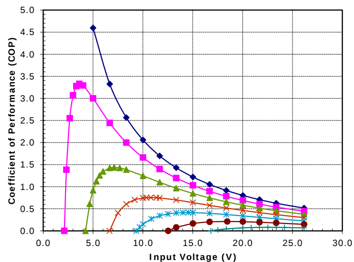
Unpotted TE-195-1.0-0.8 at a hot-side temperature of 50 °C
