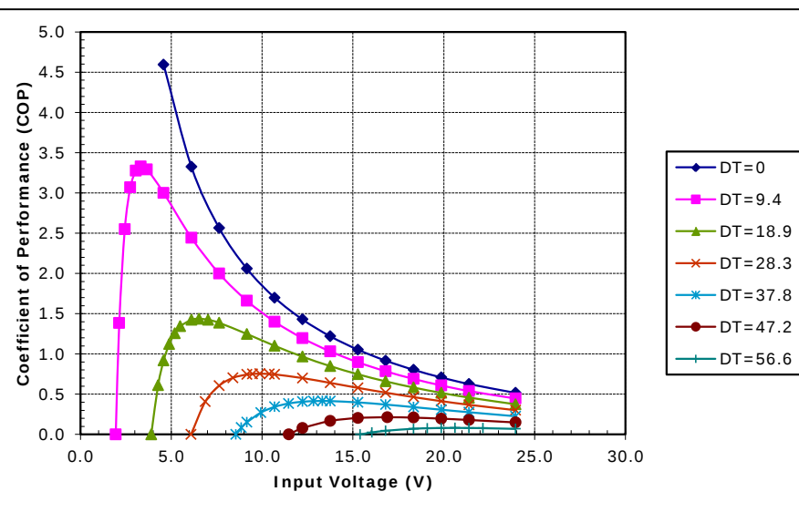
Potted TE-195-1.0-0.8 at a hot-side temperature of 30 °C
