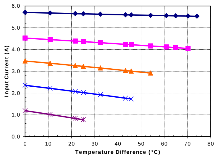
Unpotted TE-195-1.0-0.8 at a hot-side temperature of 50 °C
