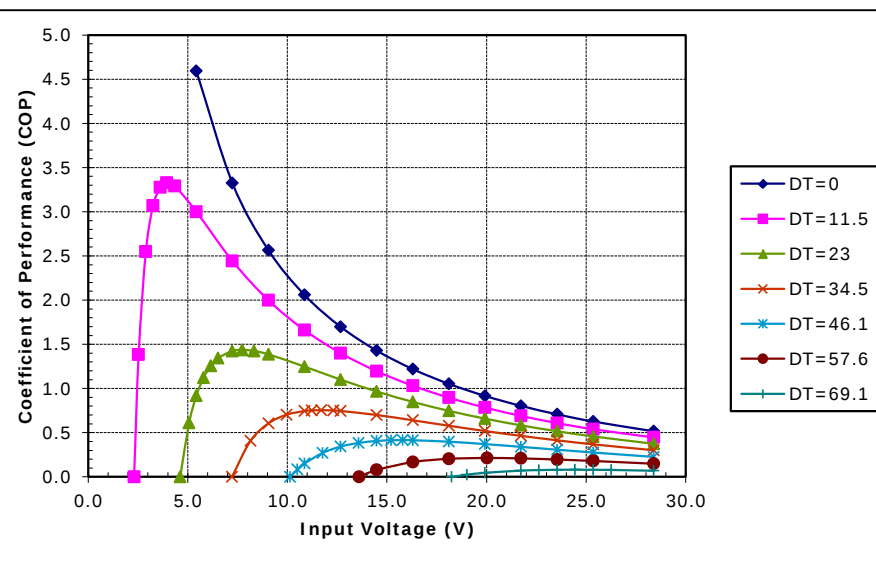
Potted TE-195-1.0-0.8 at a hot-side temperature of 70 °C
