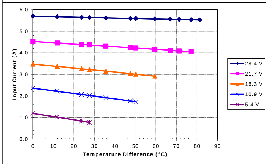
Unpotted TE-195-1.0-0.8 at a hot-side temperature of 70 °C
