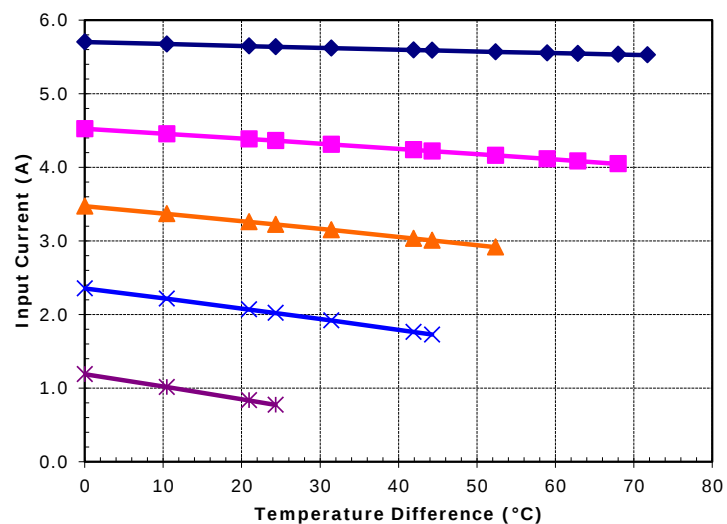
Potted TE-195-1.0-0.8 at a hot-side temperature of 50 °C
