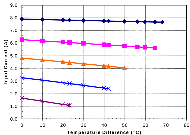
Potted TE-17-1.4-1.15 at a hot-side temperature of 50 °C
