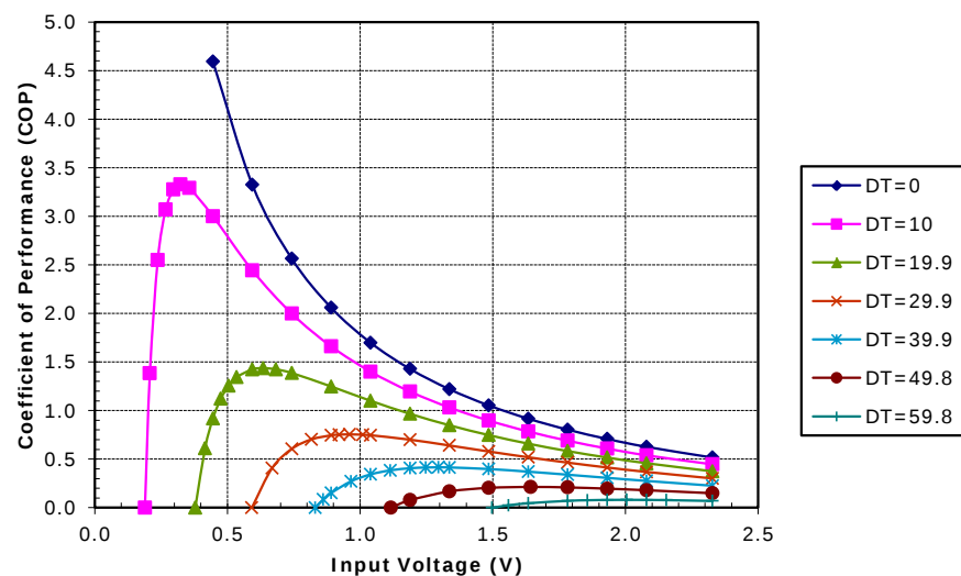
Potted TE-17-1.4-1.15 at a hot-side temperature of 50 °C
