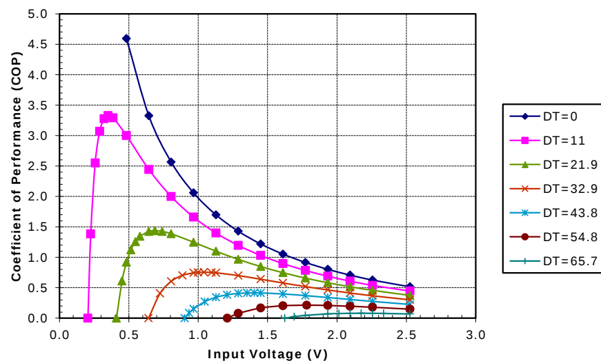
Potted TE-17-1.4-1.15 at a hot-side temperature of 70 °C
