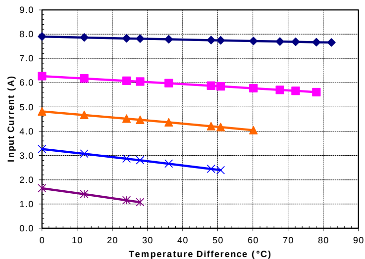
Unpotted TE-17-1.4-1.15 at a hot-side temperature of 70 °C
