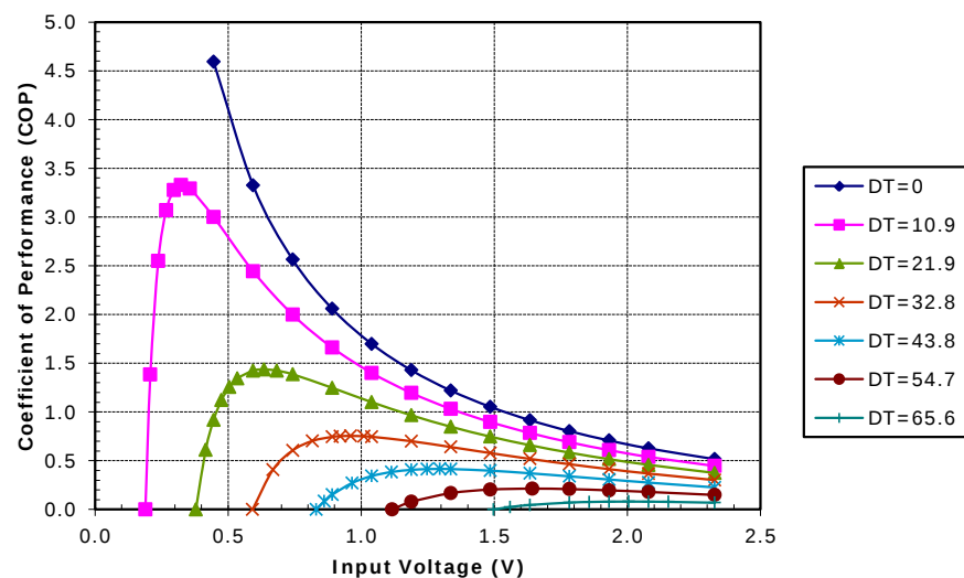
Unpotted TE-17-1.4-1.15 at a hot-side temperature of 50 °C
