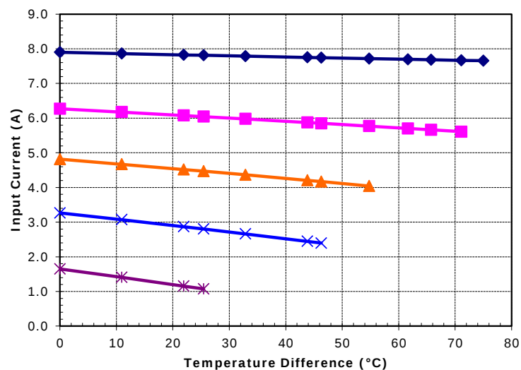
Potted TE-17-1.4-1.15 at a hot-side temperature of 70 °C
