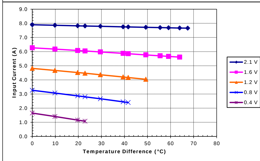
Unpotted TE-17-1.4-1.15 at a hot-side temperature of 30 °C
