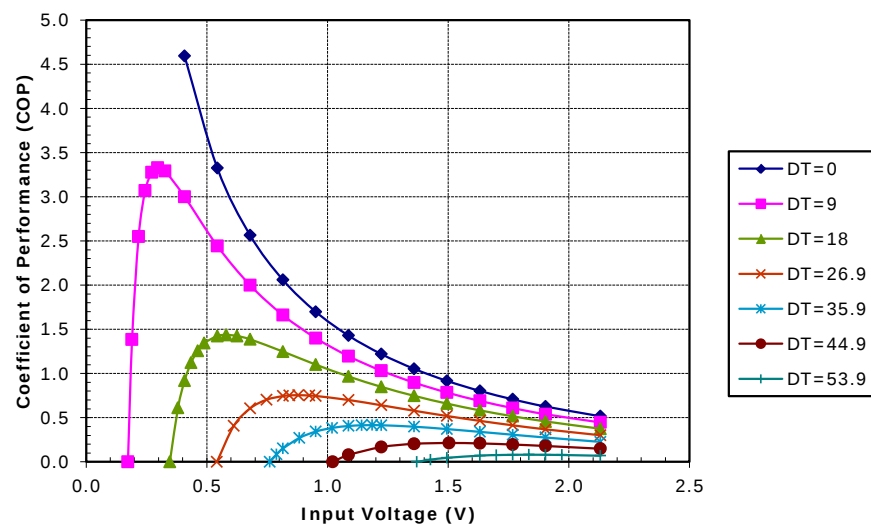
Potted TE-17-1.4-1.15 at a hot-side temperature of 30 °C
