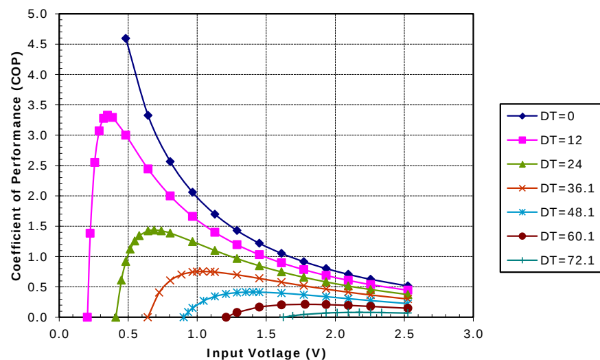
Unpotted TE-17-1.4-1.15 at a hot-side temperature of 70 °C
