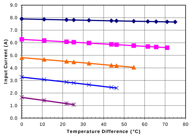
Unpotted TE-17-1.4-1.15 at a hot-side temperature of 50 °C
