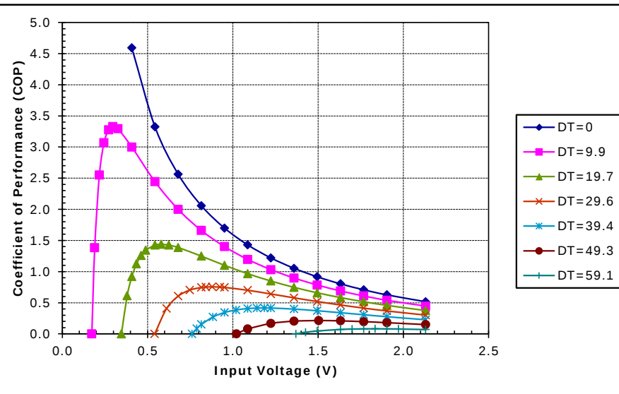
Unpotted TE-17-1.4-1.15 at a hot-side temperature of 30 °C
