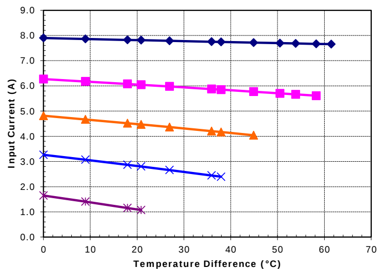
Potted TE-17-1.4-1.15 at a hot-side temperature of 30 °C
