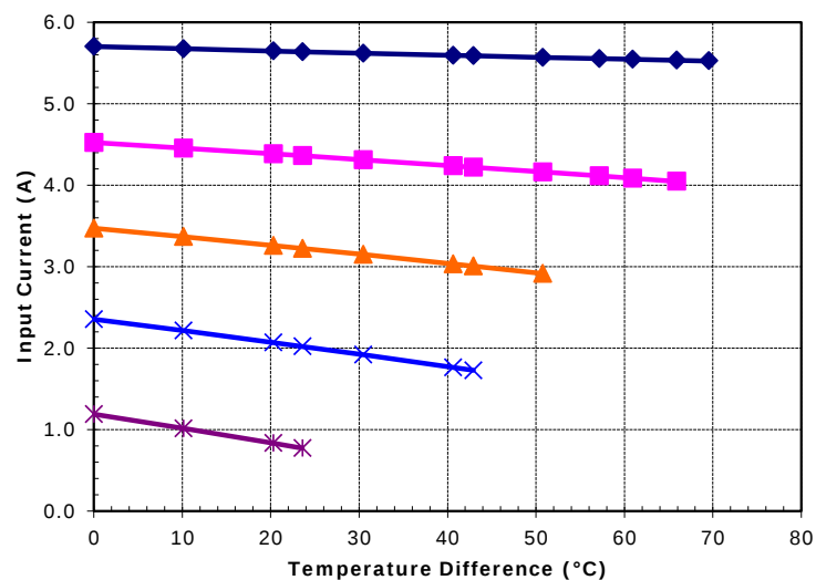
Potted CH-41-1.0-0.8 at a hot-side temperature of 70 °C
