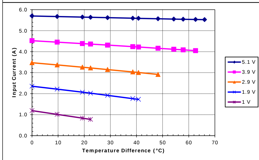
Unpotted CH-41-1.0-0.8 at a hot-side temperature of 30 °C
