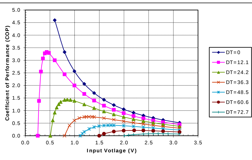
Unpotted CH-21-1.0-1.3 at a hot-side temperature of 70 °C
