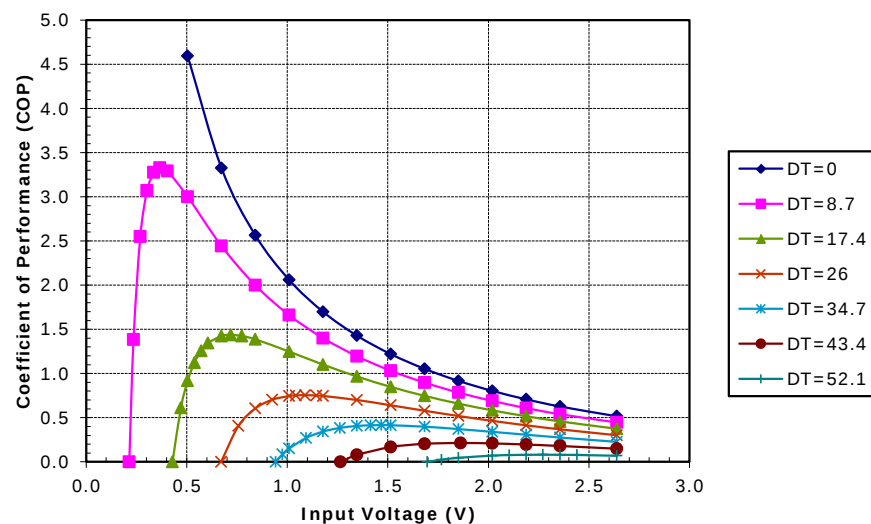
Potted CH-21-1.0-1.3 at a hot-side temperature of 30 °C
