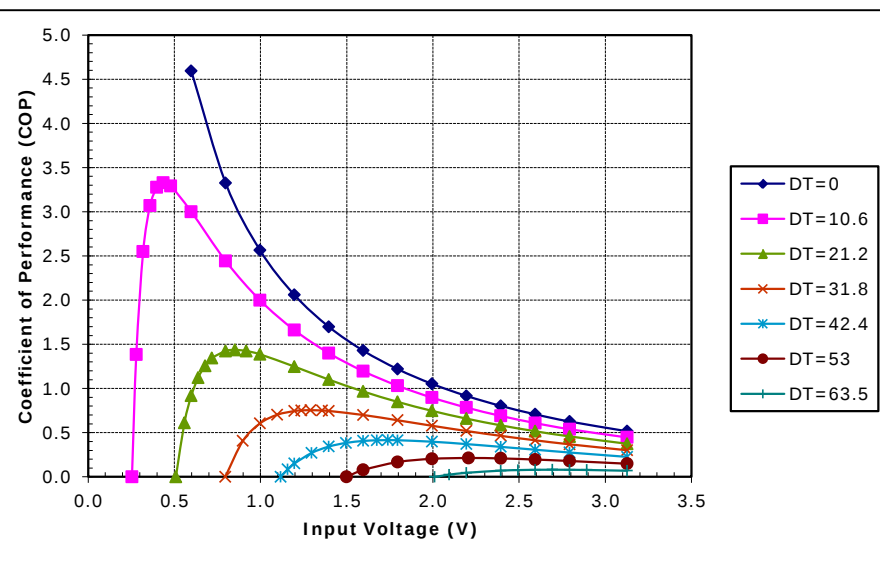
Potted CH-21-1.0-1.3 at a hot-side temperature of 70 °C
