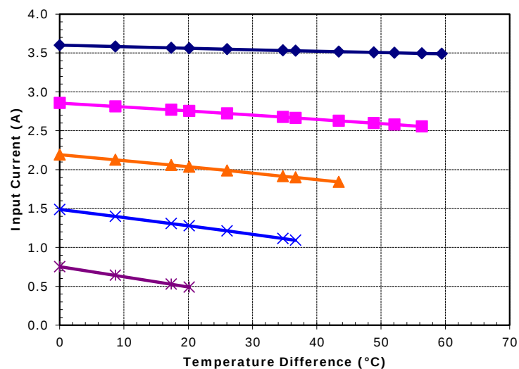
Potted CH-21-1.0-1.3 at a hot-side temperature of 30 °C
